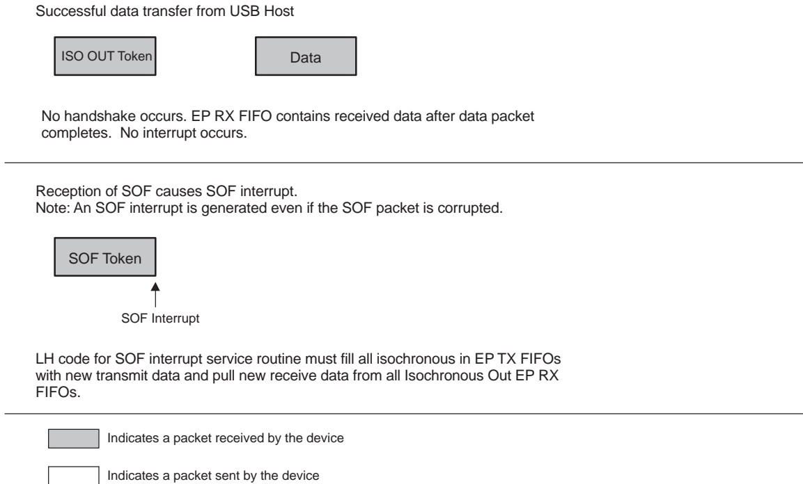
Figure 29-53. Isochronous OUT Transaction Phases and Interrupts
