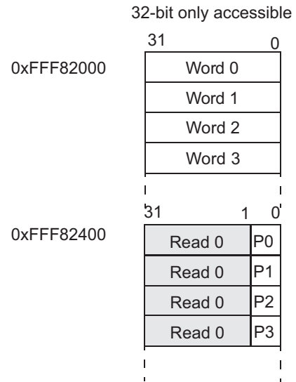
Figure 15-8. Parity Bit Mapping
