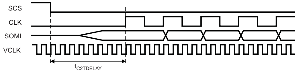
Figure 24-45. Example: t_{C2TDELAY} = 8 VCLK Cycles
