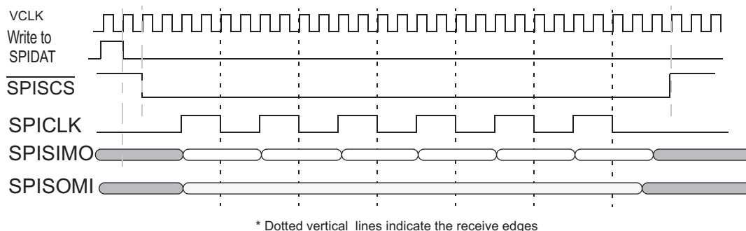
Figure 24-81. SPI/MibSPI pins during Master mode 4-pin with \overline{\text{SPISCS}} configuration.
