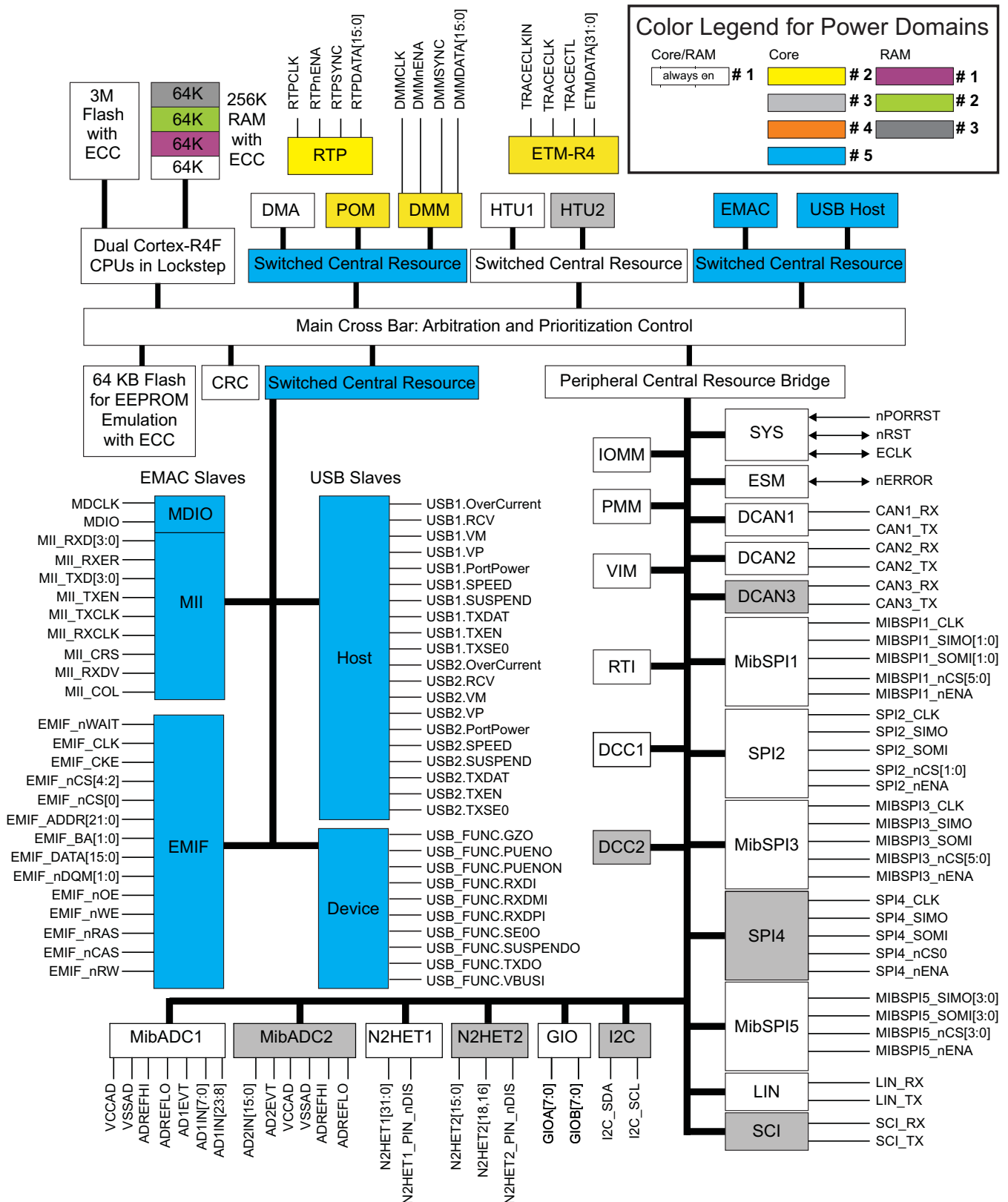
Figure 1-1. Block Diagram
