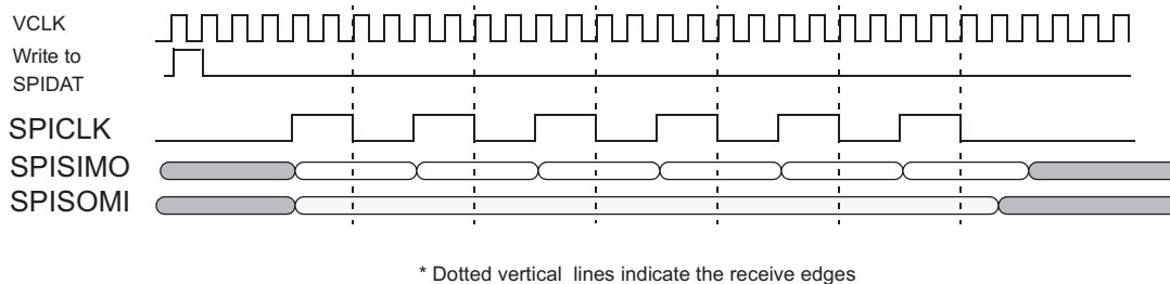
Figure 24-80. SPI/MibSPI Pins during Master mode 3-pin configuration
