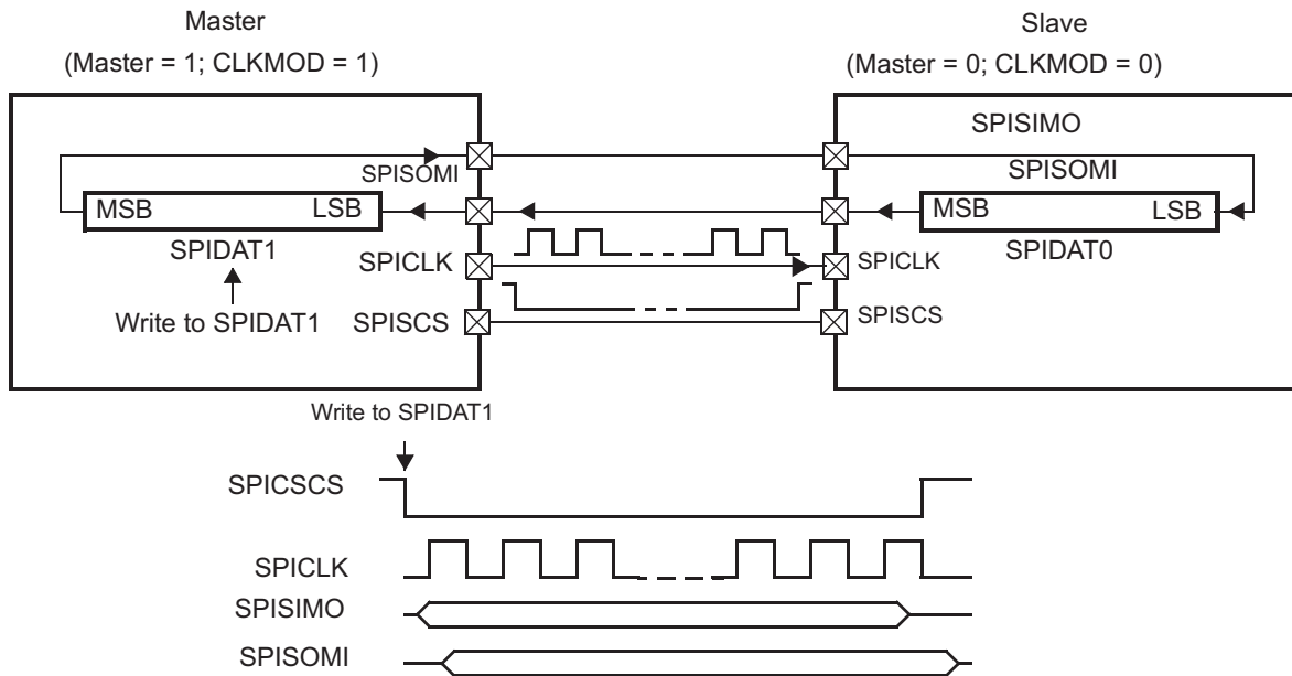
Figure 24-3. Operation with \overline{\text{SPISCS}}
