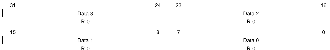
Figure 23-67. IF3 Data A Register (DCAN IF3DATA) [offset = 150h]
