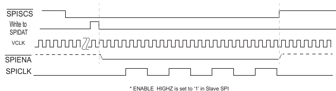
Figure 24-87. SPI/MibSPI pins during Slave mode in 5pin configuration - (Single/Multi Slave).
