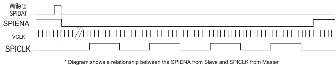
Figure 24-85. SPI/MibSPI pins during Slave mode in 4pin with \overline{\text{SPIENA}} configuration
