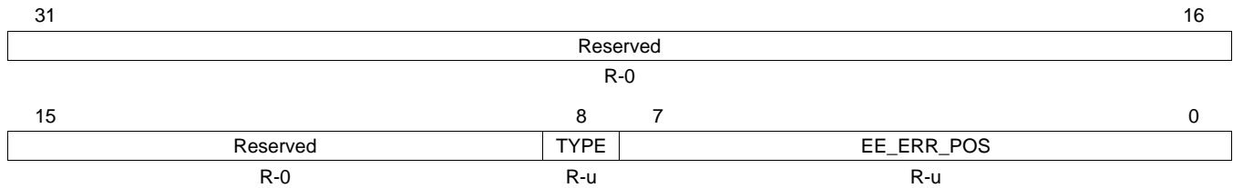
Figure 5-45. EEPROM Emulation Correctable Error Position Register (EE_COR_ERR_POS) (offset = FFF8 7318h)
