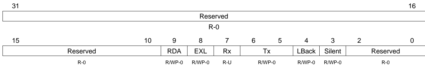
Figure 23-24. Test Register (DCAN TEST) [offset = 14h]
