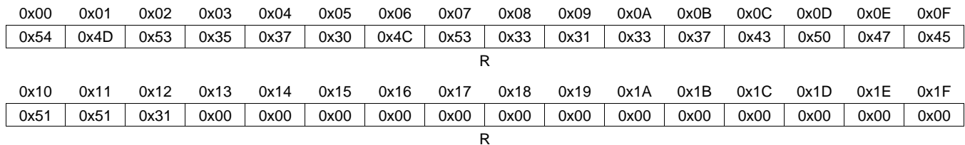
Figure 5-5. TI OTP Bank 0 Symbolization Information (F008 01E0h-F008 01FFh)
