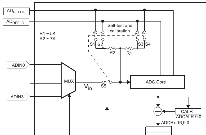
Figure 19-10. Self-Test and Calibration Logic
