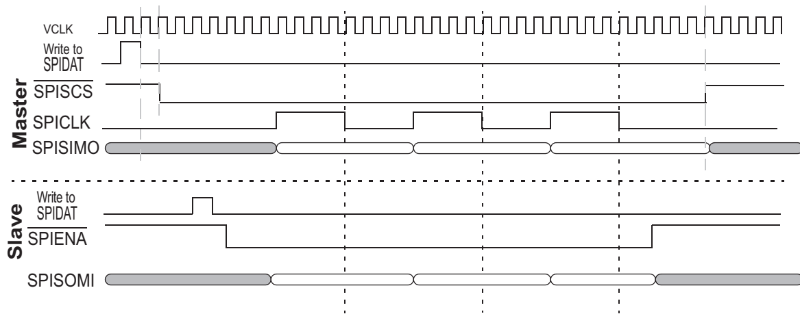
Figure 24-83. SPI/MibSPI pins during Master/Slave mode with 5-pin configuration
