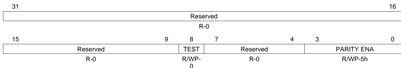
Figure 19-82. ADC Parity Control Register (ADPARCR) [offset = 180h]
