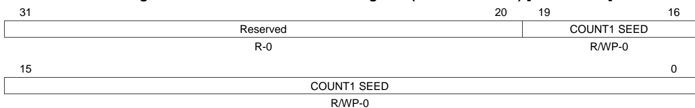
Figure 11-11. DCC Counter1 Seed Register (DCCCNT1SEED) [offset = 10h]
