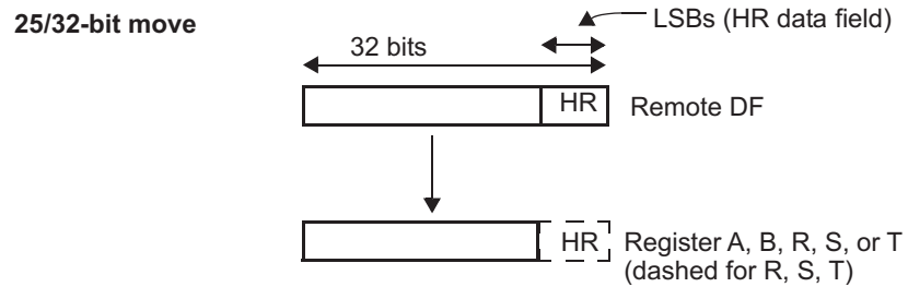
Figure 20-118. MOV32 Move Operation for REMTOREG (Case 11)
