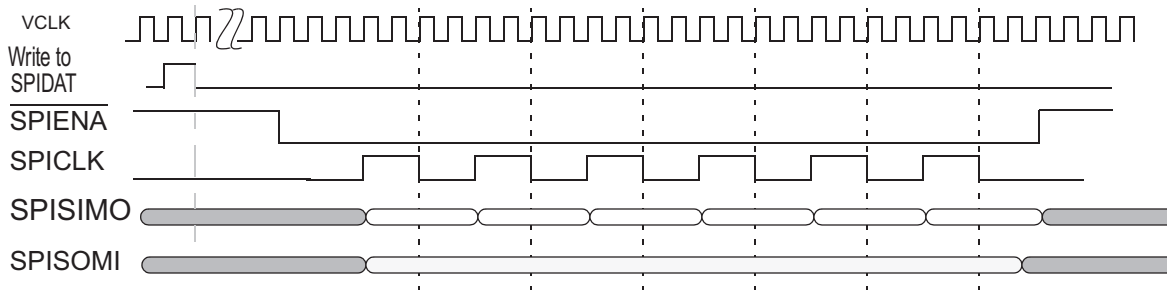
Figure 24-82. SPI/MibSPI pins during Master mode in 4pin with \overline{\text{SPIENA}} configuration
