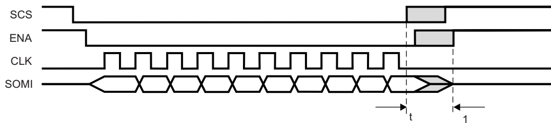
Figure 24-47. Transmit-Data-Finished-to-ENA-Inactive-Timeout
