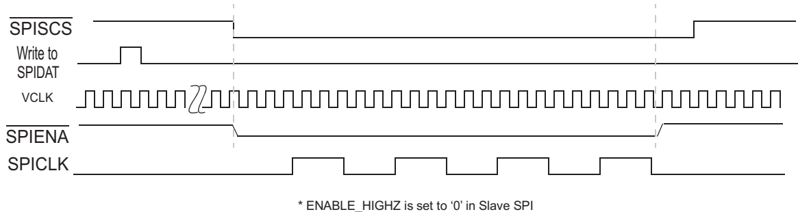
Figure 24-86. SPI/MibSPI pins during Slave mode in 5pin configuration - (Single Slave).
