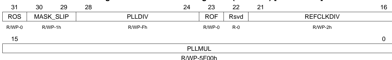
Figure 2-29. PLL Control Register 1 (PLLCTL1) [offset = 70h]
