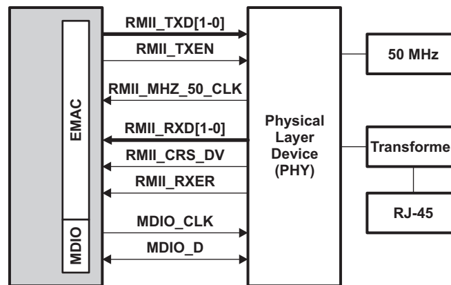
Figure 28-3. Ethernet Configuration—RMII Connections
