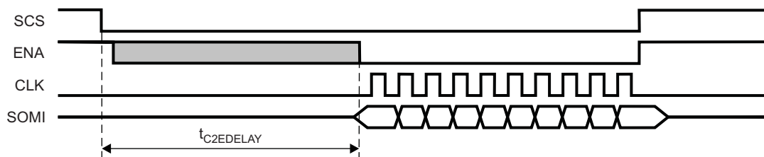
Figure 24-48. Chip-Select-Active-to-ENA-Signal-Active-Timeout
