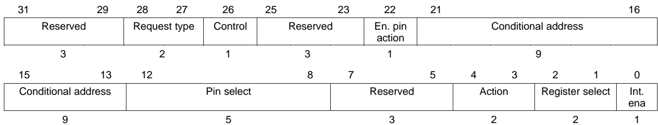
Figure 20-127. PWCNT Control Field (C31:C0)
