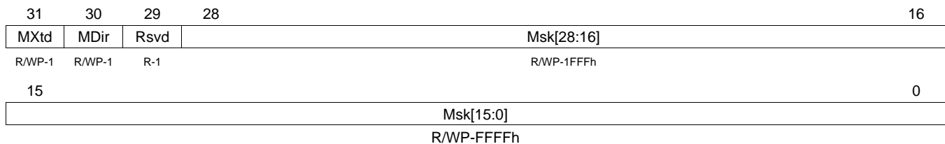
Figure 23-54. IF2 Mask Register (DCAN IF2MSK) [offset = 124h]
