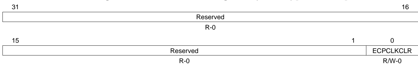
Figure 2-10. SYS Pin Control Register 6 (SYSPC6) [offset = 14h]
