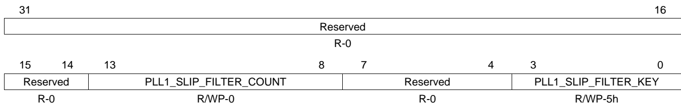
Figure 2-62. Clock Slip Register (CLKSLIP) [offset = 70h]
