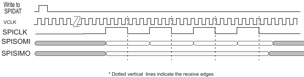
Figure 24-84. SPI/MibSPI pins during Slave mode 3-pin configuration
