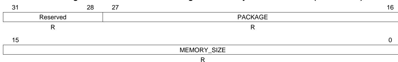
Figure 5-3. TI OTP Bank 0 Package and Memory Size Information (F008 015Ch)
