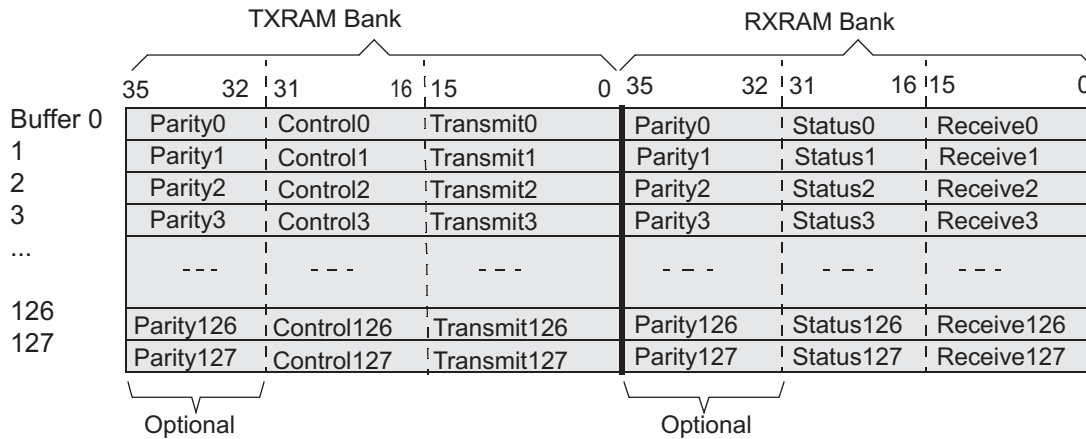
Figure 24-75. Multi-Buffer RAM Configuration
