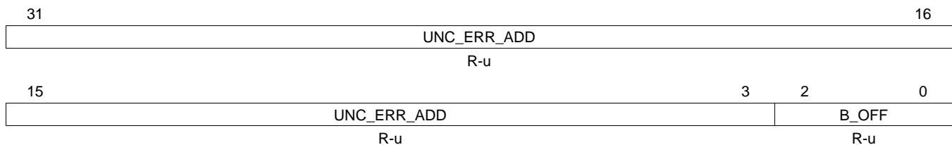
Figure 5-47. EEPROM Emulation Un-Correctable Error Address Register (EE_UNC_ERR_ADD) (offset = FFF8 7320h)
