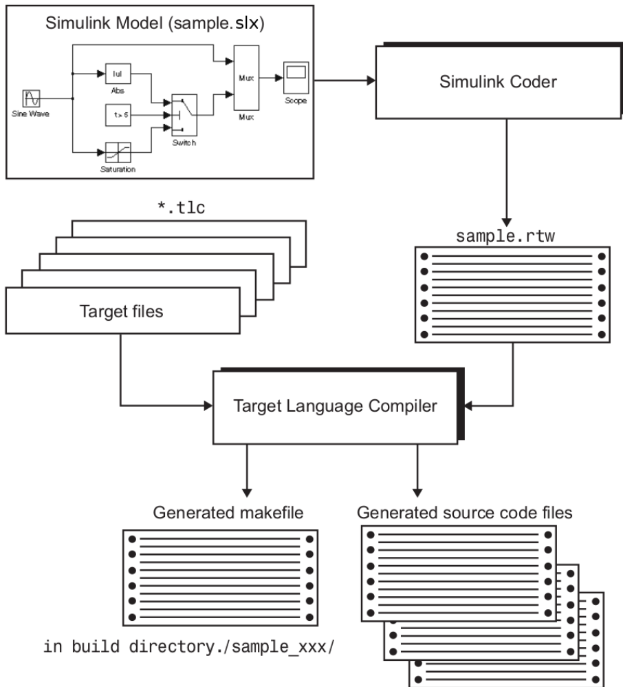
Figure 10: TLC code generation process.
