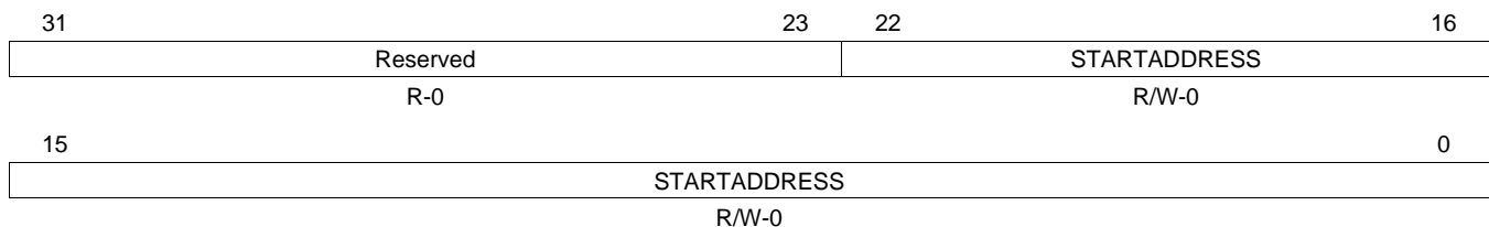
Figure 18-8. POM Overlay Region Start Register x (POMOVLSTARTx) [address = FFA04204h, FFA04214h, ..., FFA043F4h]
