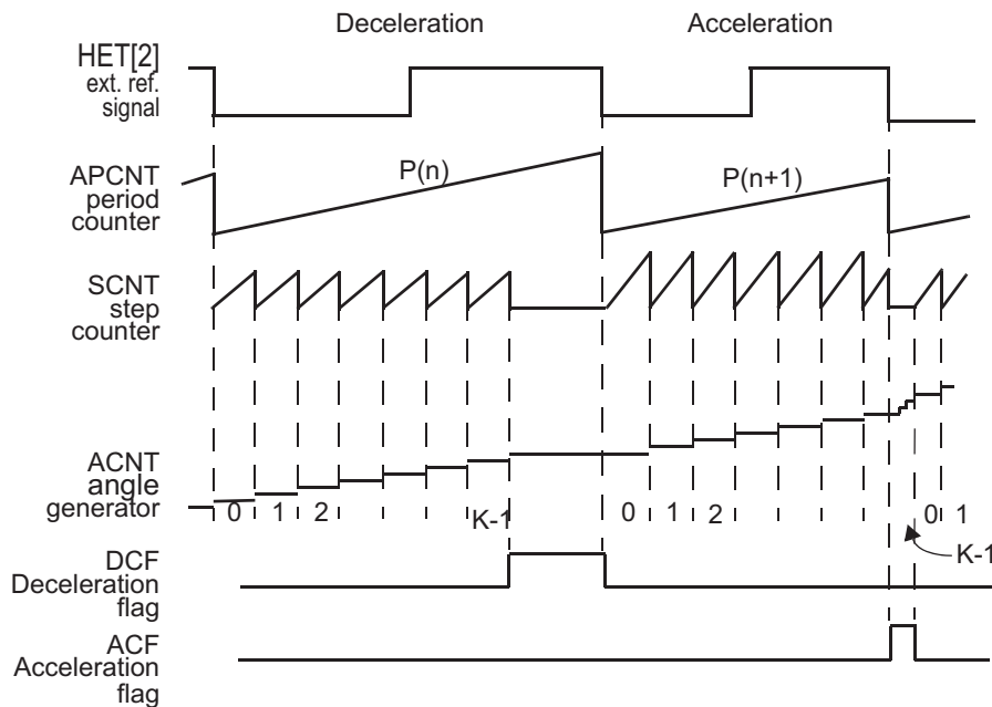
Figure 20-32. ACNT Period Variation Compensations
