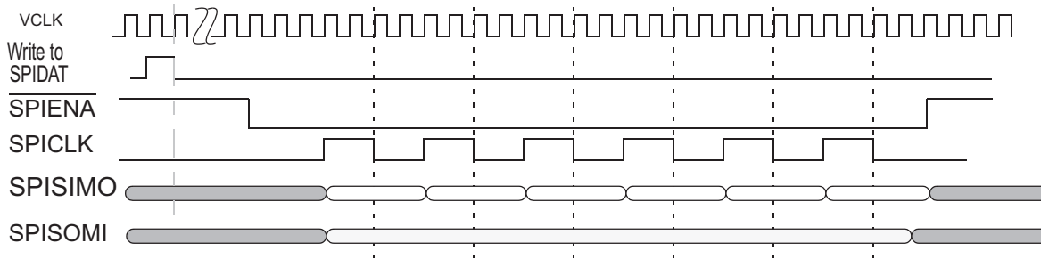
Figure 25-82. SPI/MibSPI pins during Master mode in 4pin with \overline{\text{SPIENA}} configuration
