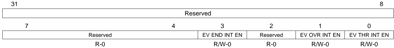
Figure 19-27. ADC Event Group Interrupt Enable Control Register (ADEVINTENA) [offset = 28h]
