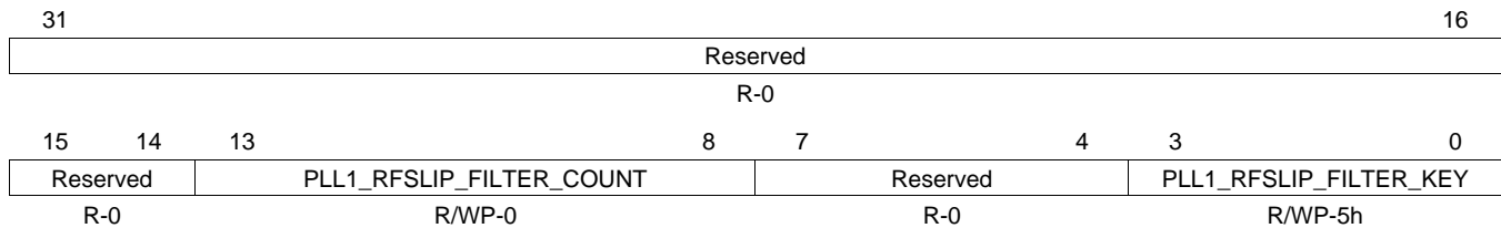
Figure 10-9. PLL Clock Slip Control Register (CLKSLIP) [offset = FFFF E170h]
