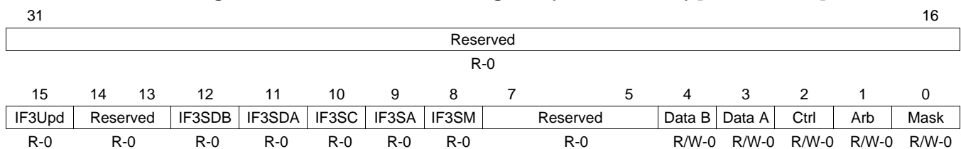
Figure 24-63. IF3 Observation Register (DCAN IF3OBS) [offset = 140h]
