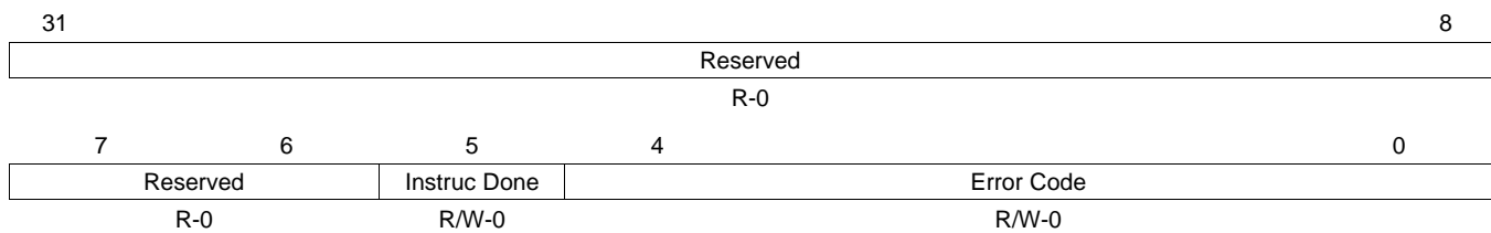
Figure 32-4. EFC Error Status Register (EFCERRSTAT) [offset = 3Ch]
