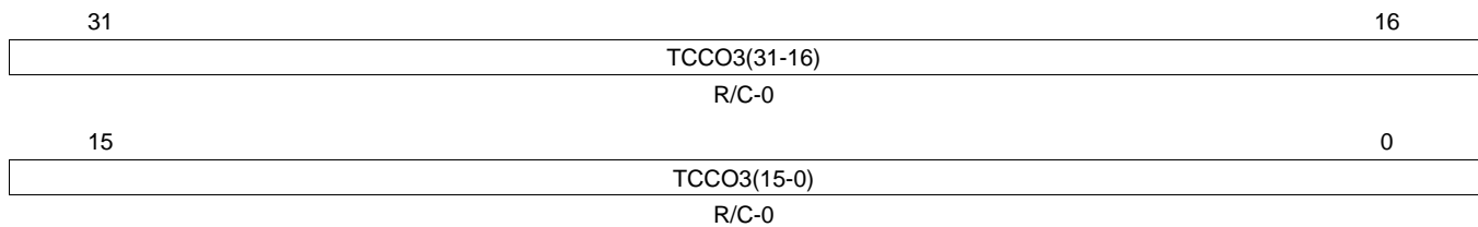
Figure 23-50. Transfer to Communication Controller Occurred 3 (TCCO3) [offset_TU = 58h]
