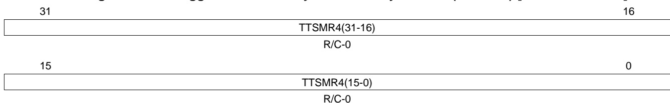
Figure 23-64. Trigger Transfer to System Memory Reset 4 (TTSMR4) [offset_TU = 9Ch]
