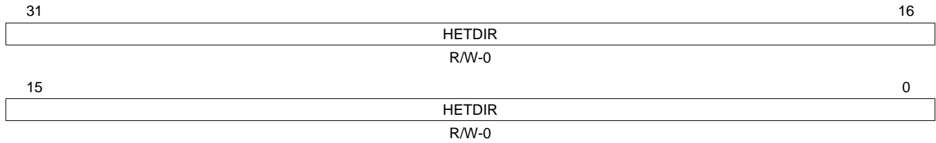
Figure 20-52. N2HET Direction Register (HETDIR)
