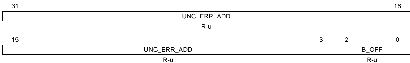
Figure 5-44. EEPROM Emulation Un-Correctable Error Address Register (EE_UNC_ERR_ADD) (offset = FFF8 7320h)
