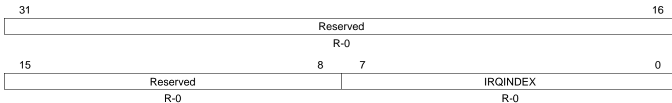
Figure 15-15. IRQ Index Offset Vector Register (IRQINDEX) [Offset = FFFF FE00h]
