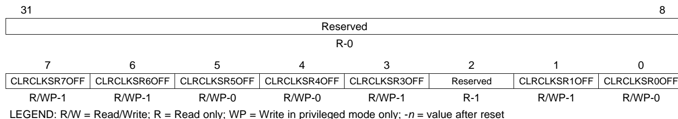
Figure 2-17. Clock Source Disable Clear Register (CSDISCLR) [offset = 38h]
