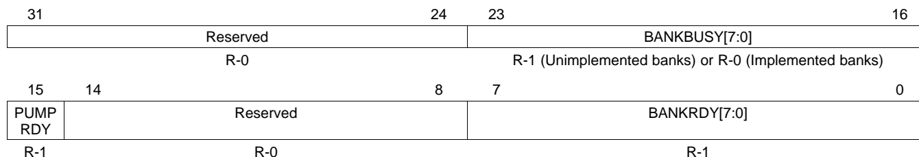
Figure 5-19. Flash Bank/Pump Ready Register (FBPRDY) (offset = FFF8 7044h)
