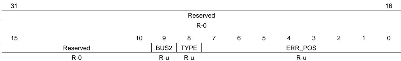
Figure 5-8. Flash Correctable Error Position Register (FCOR_ERR_POS) (offset = FFF8 7018h)
