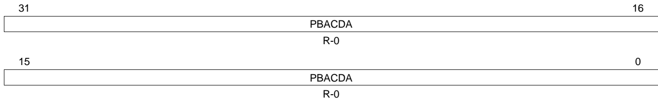
Figure 16-70. Port B Active Channel Destination Address Register (PBACDADDR) [offset = 19Ch]
