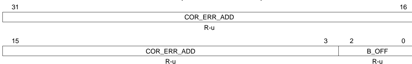
Figure 5-41. EEPROM Emulation Correctable Error Address Register (EE_COR_ERR_ADD) (offset = FFF8 7314h)
