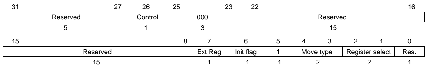
Figure 20-83. ADM32 Control Field (C31:C0)
