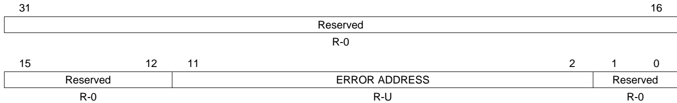
Figure 19-83. ADC Parity Error Address Register (ADPARADDR) [offset = 184h]
