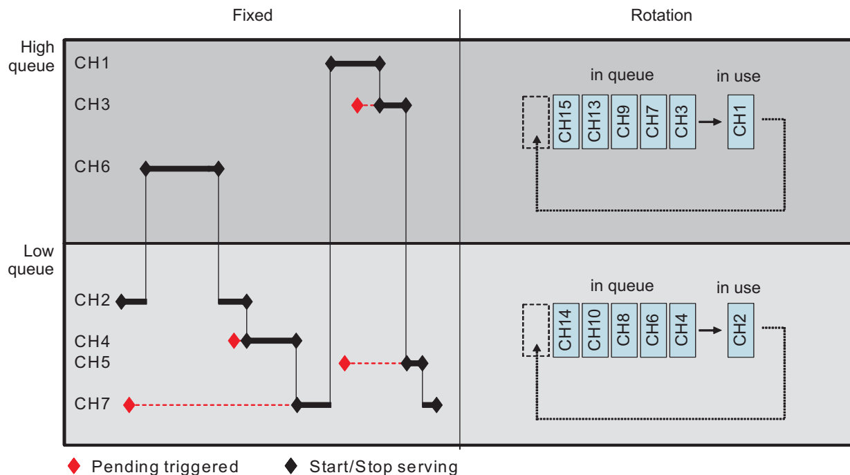
Figure 16-10. Example of Priority Queues
