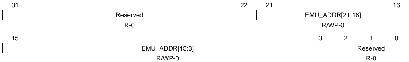
Figure 5-28. EEPROM Emulation Address Register (FEMU_ADDR) (offset = FFF8 7068h)
