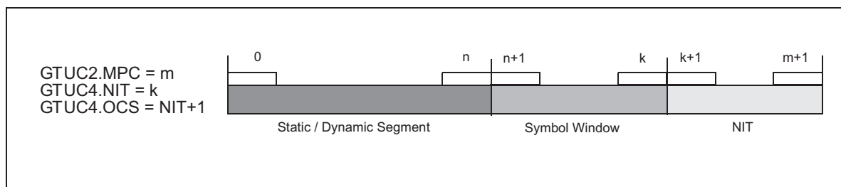
Figure 23-13. Configuration of NIT Start and Offset Correction Start
