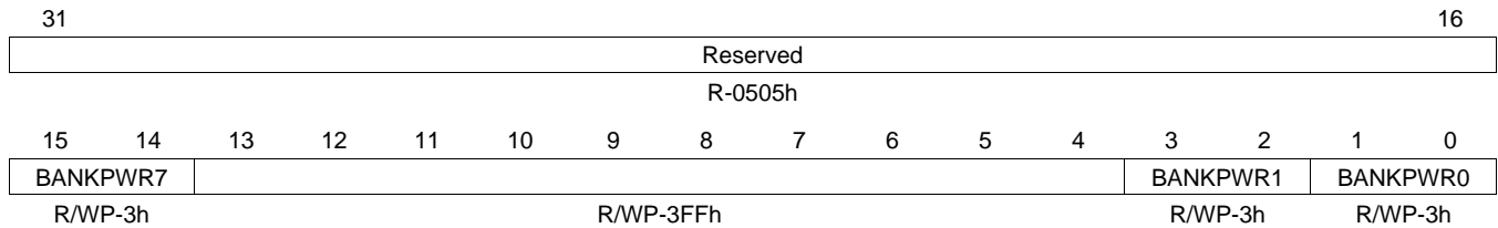
Figure 5-18. Flash Bank Fallback Power Register (FBFALLBACK) (offset = FFF8 7040h)
