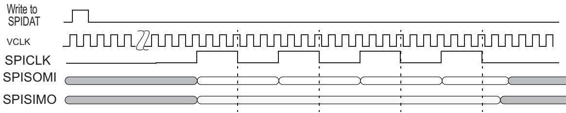
Figure 25-84. SPI/MibSPI pins during Slave mode 3-pin configuration
