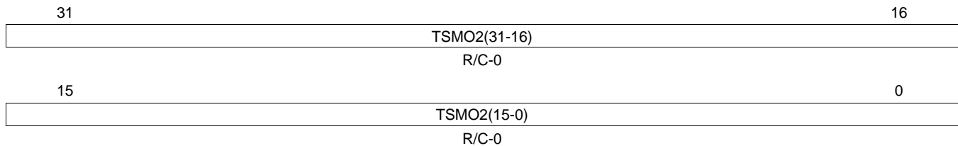
Figure 23-45. Transfer to System Memory Occurred 2 (TSMO2) [offset_TU = 44h]
