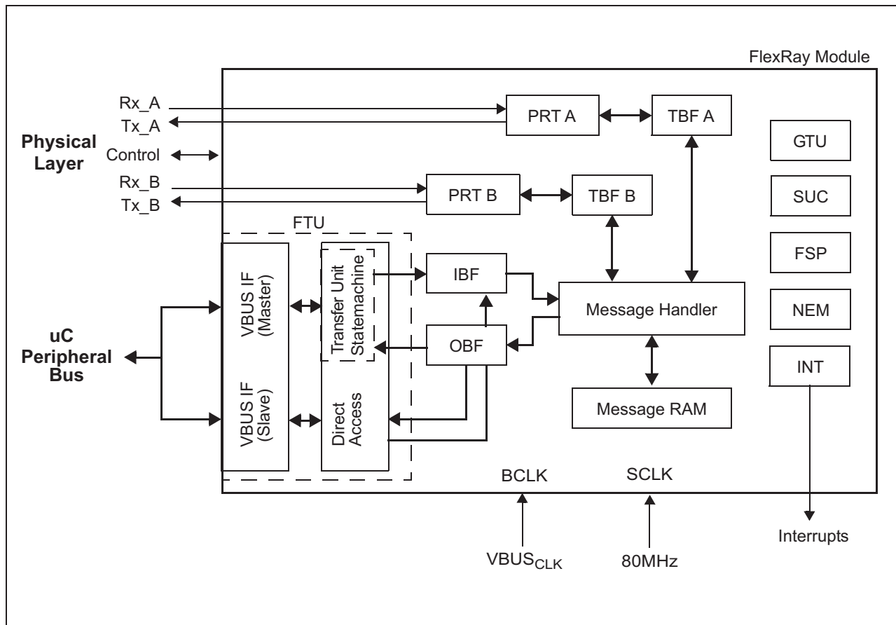
Figure 23-1. Block Diagram
