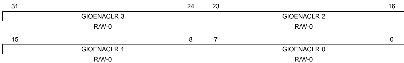
Figure 22-9. GIO Interrupt Enable Clear Register (GIOENACLR) [address = FFF7 BC14h]
