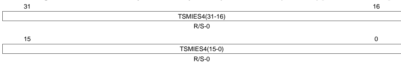
Figure 23-95. Transfer to System Memory Interrupt Enable Set 4 (TSMIES4) [offset_TU = 118h]
