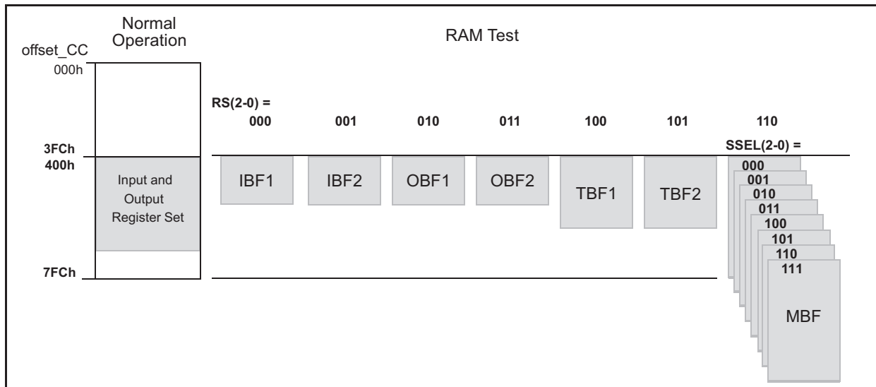
Figure 23-110. Test Mode Access to Communication Controller RAM Blocks
