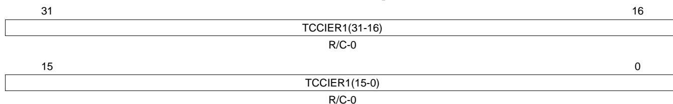
Figure 23-98. Transfer to Communication Controller Interrupt Enable Reset 1 (TCCIER1) [offset_TU = 124h]
