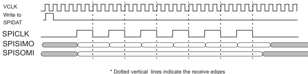
Figure 25-80. SPI/MibSPI Pins during Master mode 3-pin configuration
