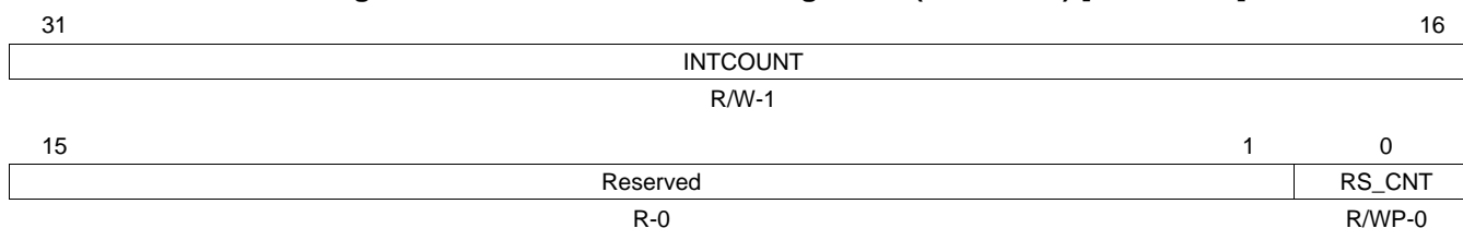
Figure 8-3. STC Global Control Register 0 (STCGCR0) [offset = 00]
