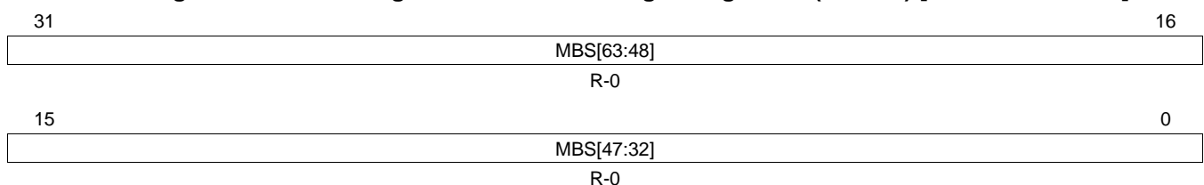
Figure 23-171. Message Buffer Status Changed Register 2 (MBSC2) [offset_CC = 344h]
