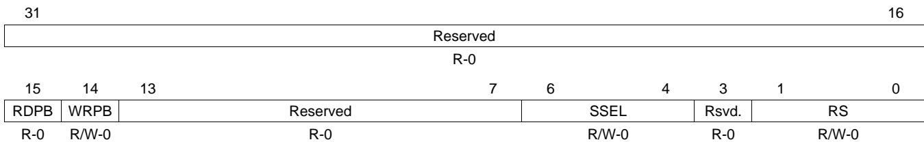
Figure 23-109. Test Register 2 (TEST2) [offset_CC = 14h]
