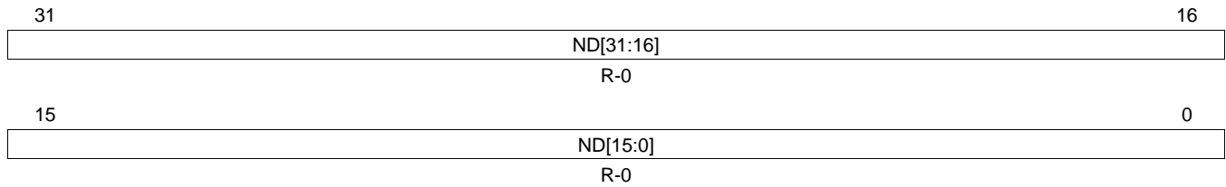
Figure 23-168. New Data Register 1 (NDAT1) [offset_CC = 330h]
