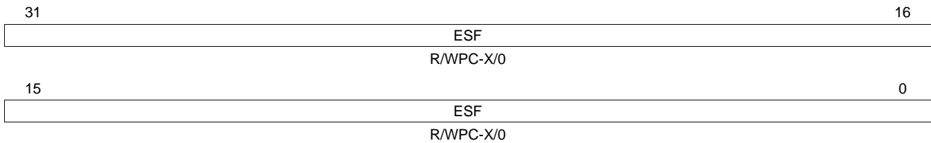
Figure 12-19. ESM Status Register 3 (ESMSR3) [offset = FFFF F520h]
