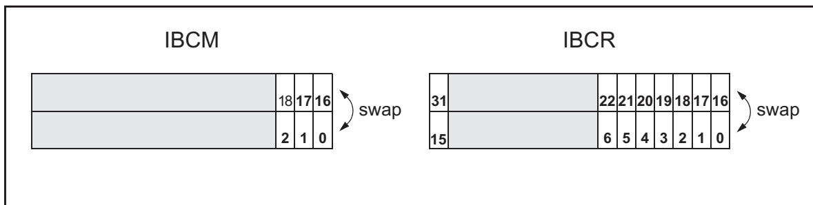
Figure 23-21. Swapping of IBCM and IBCR Bits
