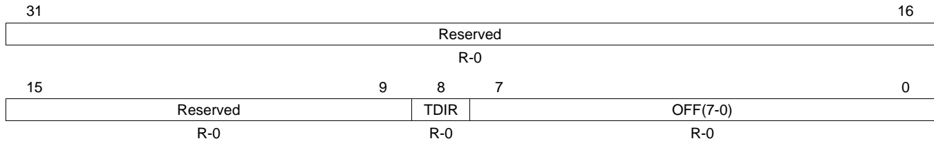
Figure 23-52. Transfer Occurred Offset (TOOFF) [offset_TU = 60h]
