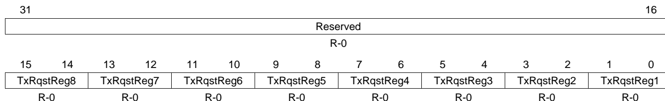
Figure 24-27. Transmission Request X Register (DCAN TXRQ X) [offset = 84h]
