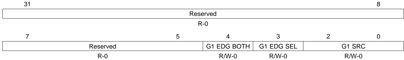
Figure 19-25. ADC Group1 Trigger Source Select Register (ADG1SRC) [offset = 20h]
