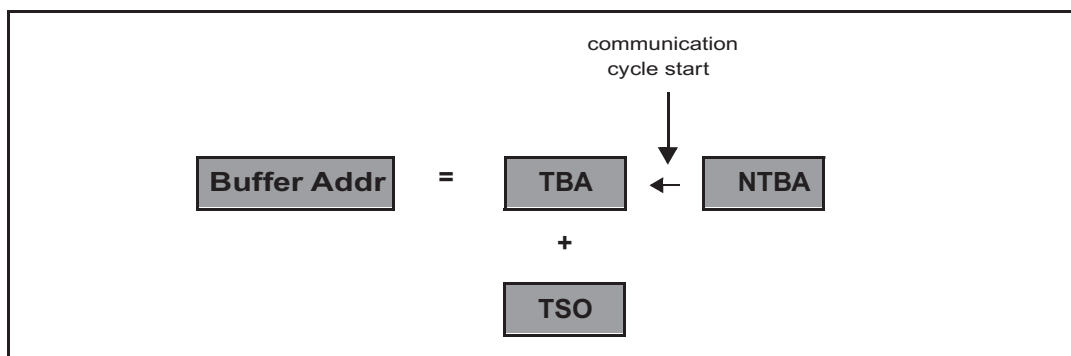
Figure 23-11. Transfer Start Address to Message Buffer Number Assignment
