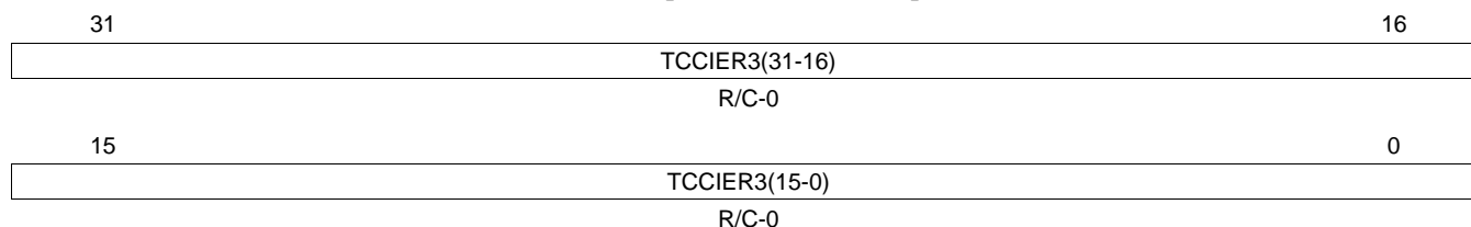
Figure 23-102. Transfer to Communication Controller Interrupt Enable Reset 3 (TCCIER3) [offset_TU = 134h]
