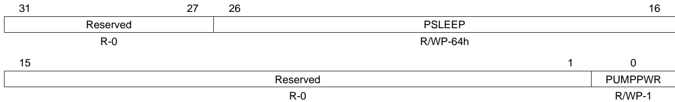
Figure 5-20. Flash Pump Access Control Register 1 (FPAC1) (offset = FFF8 7048h)
