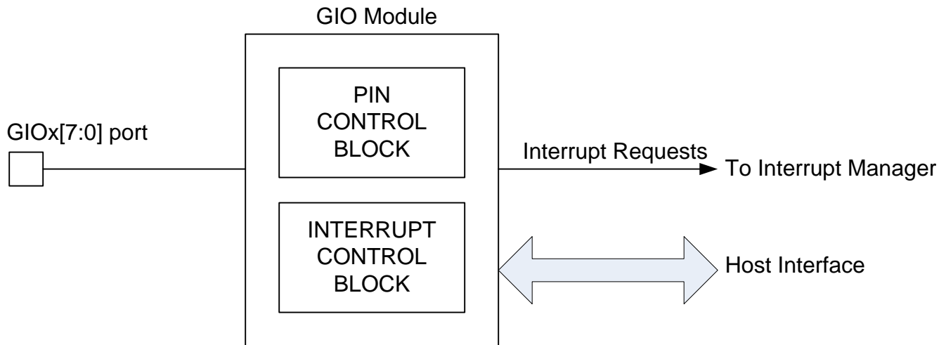
Figure 22-1. GIO Block Diagram
