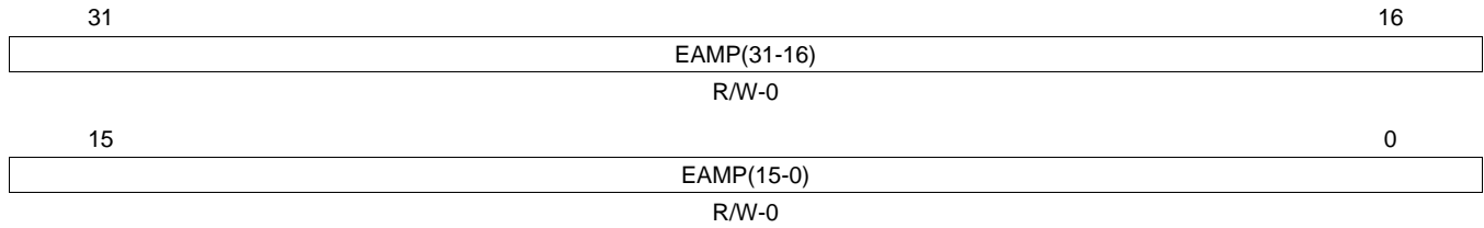
Figure 23-43. End Address of Memory Protection (EAMP) [offset_TU = 34h]
