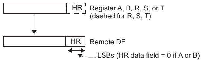
Figure 20-118. MOV32 Move Operation for REMTOREG (Case 11)
