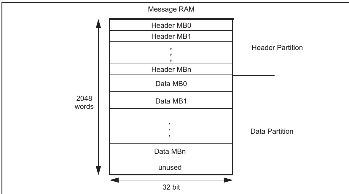
Figure 23-25. Configuration Example of Message Buffers in the Message RAM
