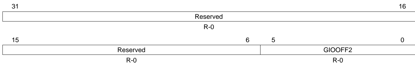
Figure 22-14. GIO Offset 2 Register (GIOFF2) [address = FFF7 BC28h]
