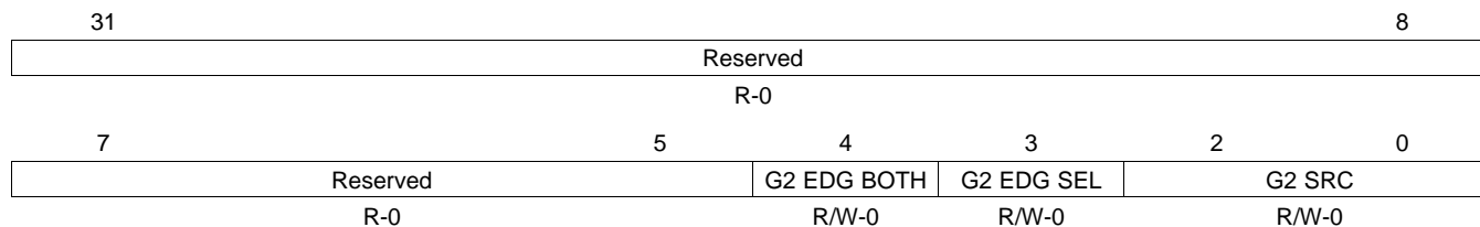
Figure 19-26. ADC Group2 Trigger Source Select Register (ADG2SRC) [offset = 24h]
