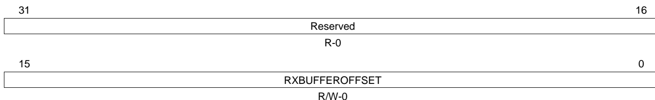
Figure 29-63. Receive Buffer Offset Register (RXBUFFEROFFSET)
