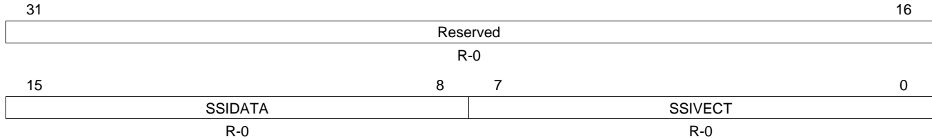
Figure 2-57. Software Interrupt Vector Register (SSIVEC) [offset = F4h]
