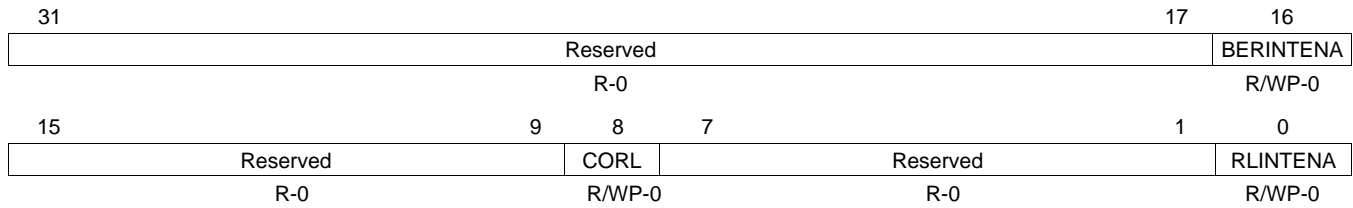
Figure 21-21. Request Lost and Bus Error Control Register (HTU RLBECTRL) [offset = 20h]
