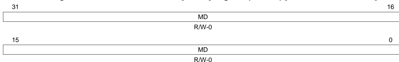
Figure 23-175. Write Data Section [1..64] Register (WRDSn) [offset_CC = 400h-4FCh]
