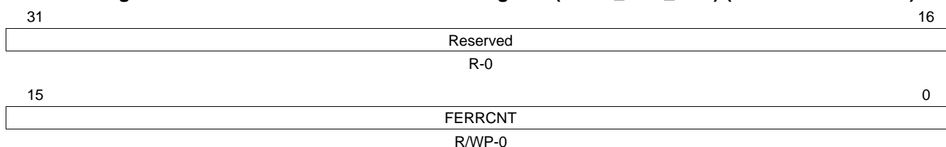
Figure 5-6. Flash Correctable Error Count Register (FCOR_ERR_CNT) (offset = FFF8 7010h)
