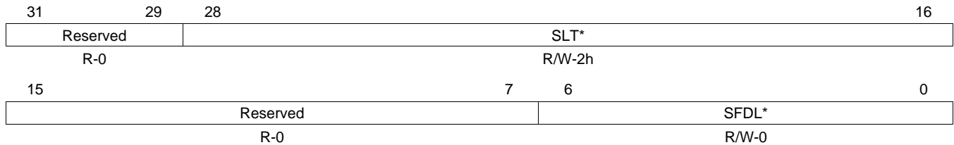
Figure 23-129. MHD Configuration Register (MHDC) [offset_CC = 98h]
