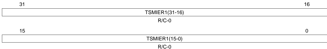
Figure 23-90. Transfer to System Memory Interrupt Enable Reset 1 (TSMIER1) [offset_TU = 104h]
