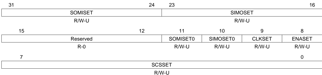
Figure 25-35. SPI Pin Control Register 4 (SPIPC4) [offset = 24h]
