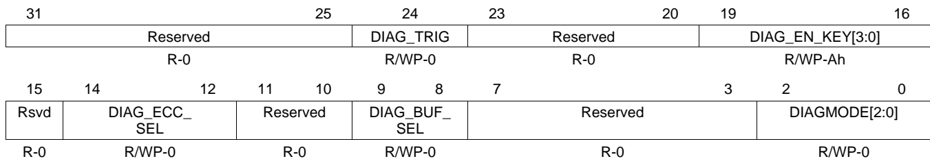
Figure 5-29. Diagnostic Control Register (FDIAGCTRL) (offset = FFF8 706Ch)
