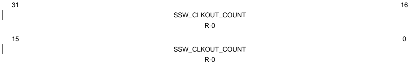
Figure 10-13. SSW PLL BIST Control Register 3 (SSWPLL3) [offset = 2Ch]
