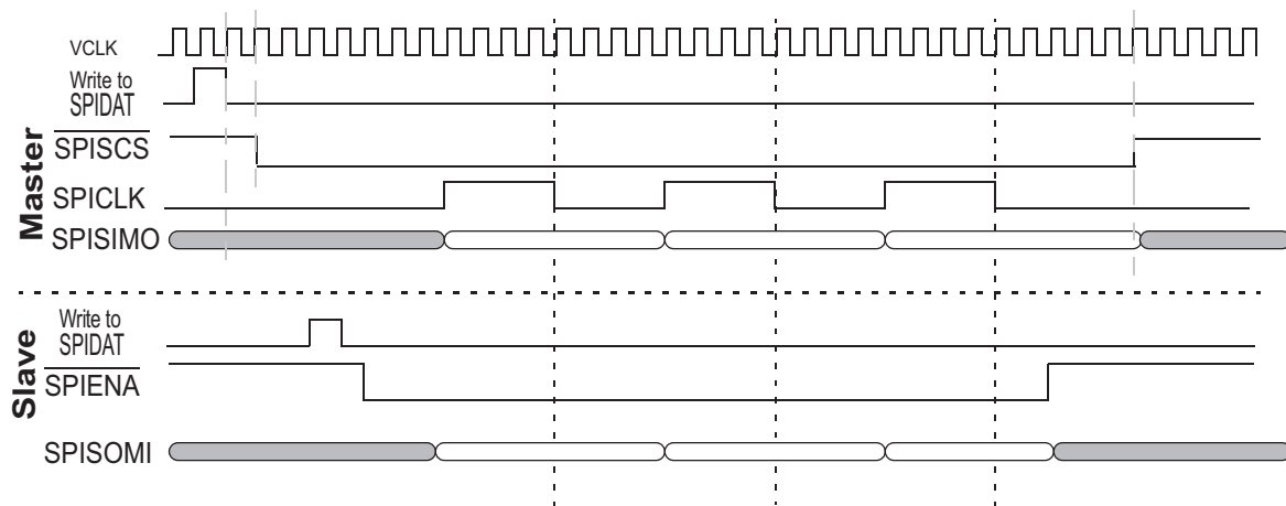
Figure 25-83. SPI/MibSPI pins during Master/Slave mode with 5-pin configuration
