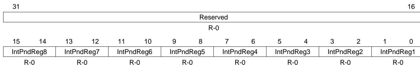
Figure 24-37. Interrupt Pending X Register (DCAN INTPND X) [offset = ACh]
