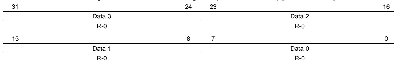
Figure 24-67. IF3 Data A Register (DCAN IF3DATA) [offset = 150h]
