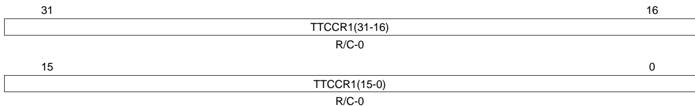
Figure 23-66. Trigger Transfer to Communication Controller Reset 1 (TTCCR1) [offset_TU = A4h]
