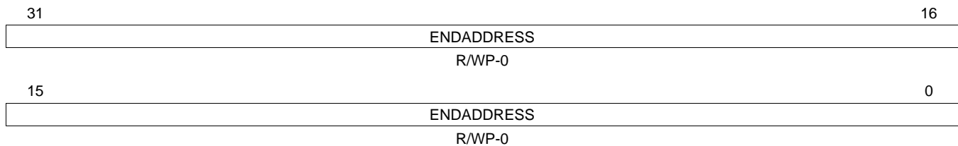
Figure 16-81. DMA Memory Protection Region 2 End Address Register (DMAMPR2E) [offset = 1CCh]
