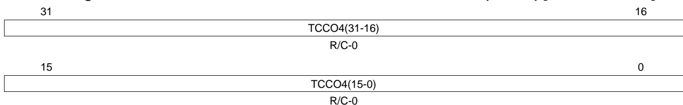
Figure 23-51. Transfer to Communication Controller Occurred 4 (TCCO4) [offset_TU = 5Ch]
