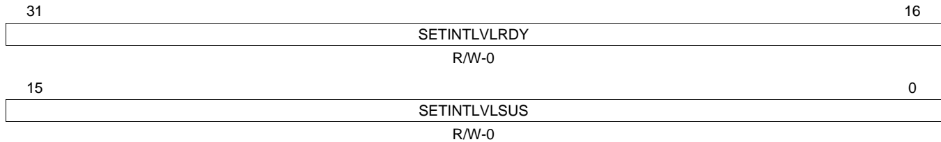
Figure 25-57. Transfer Group Interrupt Level Set Register (TGITLVST) [offset = 7Ch]
