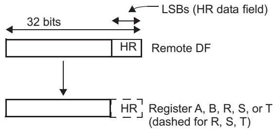
Figure 20-118. MOV32 Move Operation for REMTOREG (Case 11)
