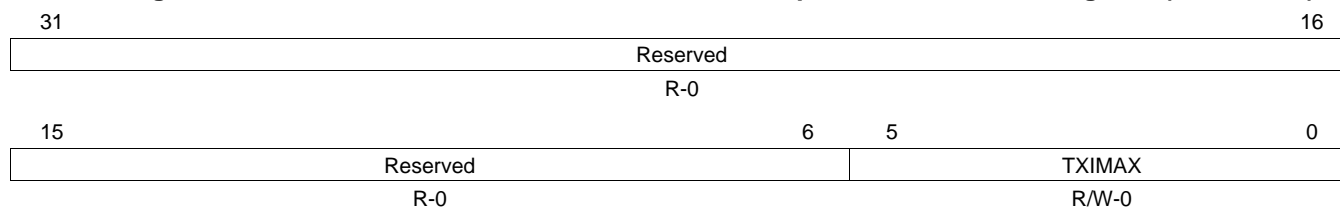
Figure 29-24. EMAC Control Module Transmit Interrupts Per Millisecond Register (C0TXIMAX)
