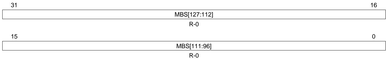
Figure 23-169. Message Buffer Status Changed Register 4 (MBSC4) [offset_CC = 34Ch]
