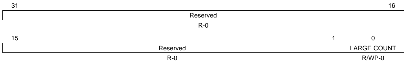
Figure 25-66. DMA Large Count Register (DMACNTLEN) [offset = 118h]
