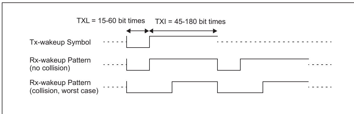
Figure 23-16. Timing of Wake Up Pattern
