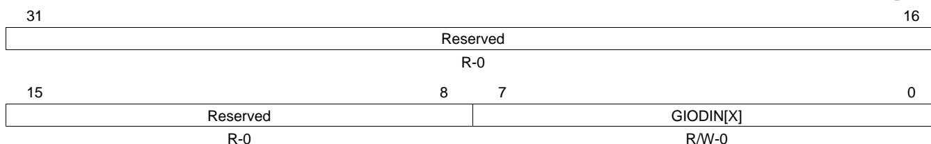
Figure 22-18. GIO Data Input Registers [A-H][7:0] (GIODIN[A-H]) [address = FFF7BC38h, FFF7BC58h, FFF7BC78h, FFF7BC98h, FFF7BCB8h, FFF7BCD8h, FFF7BCF8h, FFF7BD18h]
