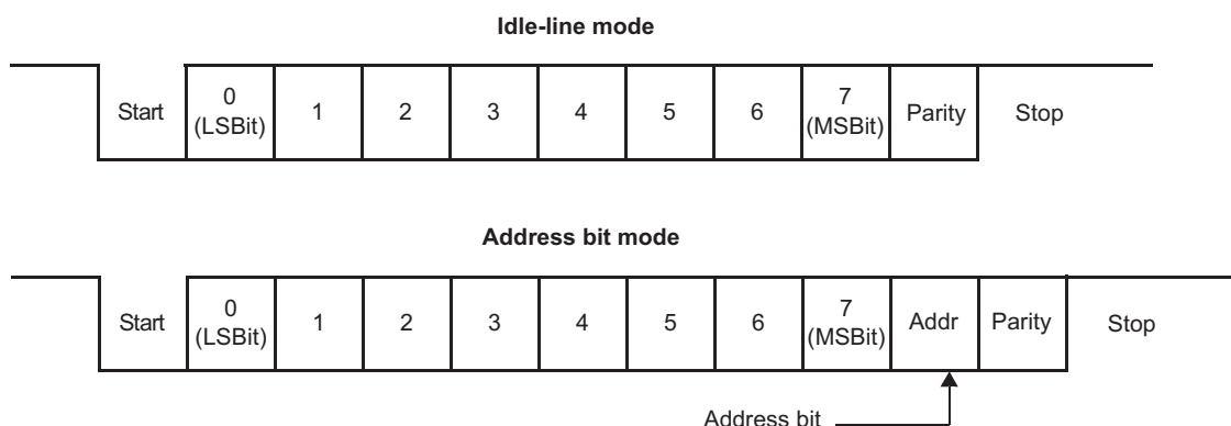
Figure 26-3. Typical SCI Data Frame Formats
