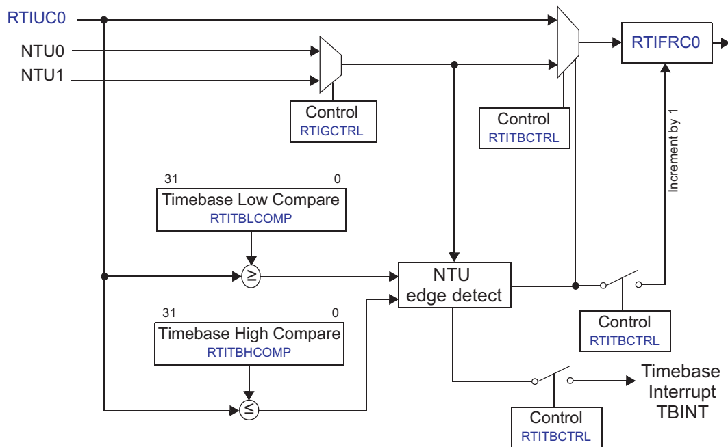
Figure 13-4. Timebase Control
