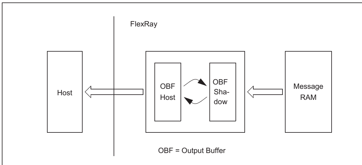
Figure 23-22. Double Buffer Structure Output Buffer
