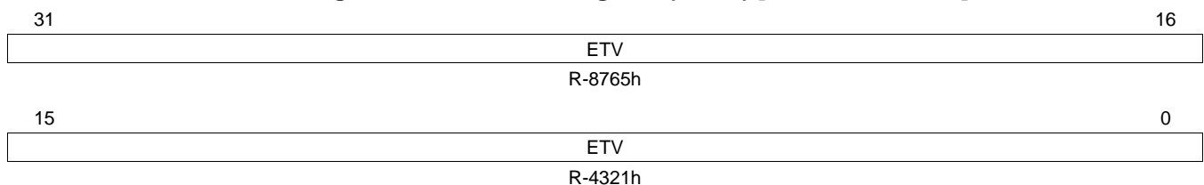
Figure 23-174. Endian Register (ENDN) [offset_CC = 3F4h]
