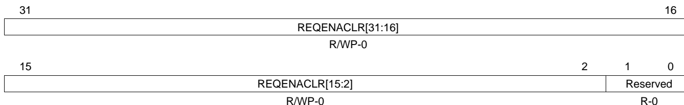
Figure 15-26. Interrupt Enable Clear Register 0 (REQENACLR0) [offset = FFFF FE40h]
