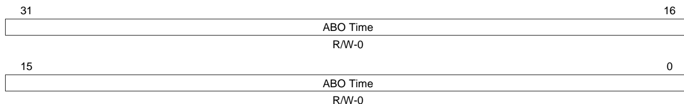
Figure 24-26. Auto-Bus-On Time Register (DCAN ABOTR) [offset = 80h]
