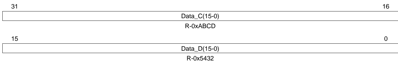
Figure 23-33. Global Static Number 1 (GSN1) [offset_TU = 04h]
