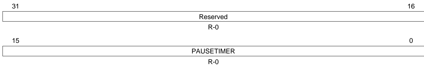
Figure 29-80. Transmit Pause Timer Register (TXPAUSE)
