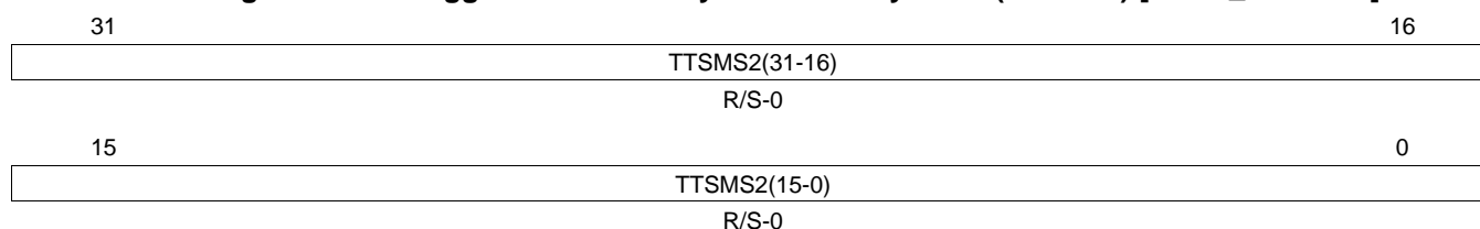
Figure 23-59. Trigger Transfer to System Memory Set 2 (TTSMS2) [offset_TU = 88h]
