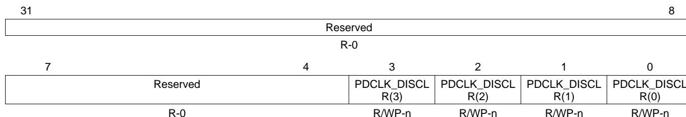
Figure 3-7. Power Domain Clock Disable Clear Register (PDCLKDISCLRREG) [offset = 28h]
