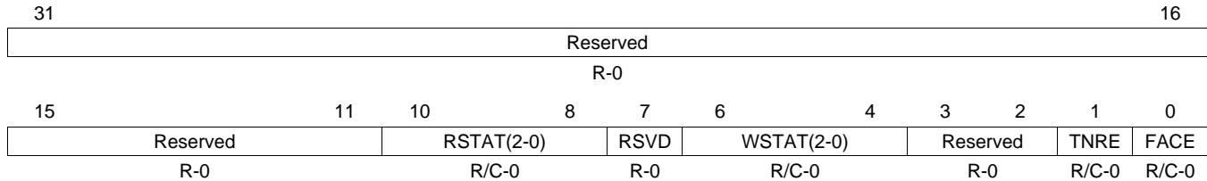
Figure 23-56. Transfer Error Interrupt Enable Reset (TEIRER) [offset_TU = 7Ch]
