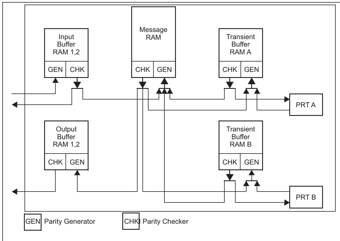
Figure 23-29. Parity Generation and Check
