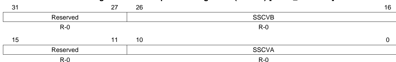
Figure 23-122. Stop Watch Register 2 (STPW2) [offset_CC = 50h]
