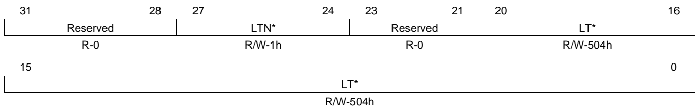
Figure 23-124. SUC Configuration Register 2 (SUCC2) [offset_CC = 84h]
