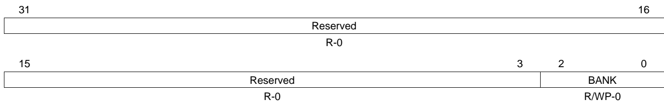
Figure 5-22. Flash Module Access Control Register (FMAC) [offset = FFF8 7050h]
