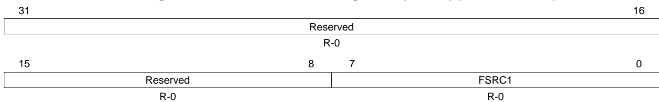
Figure 7-11. Fail Status Count Register 1 (FSRC1) [offset = 019Ch]
