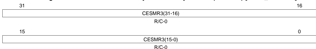
Figure 23-86. Clear on Event to System Memory Reset 3 (CESMR3) [offset_TU = F4h]
