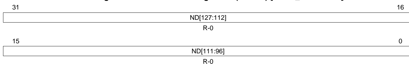
Figure 23-165. New Data Register 4 (NDAT4) [offset_CC = 33Ch]
