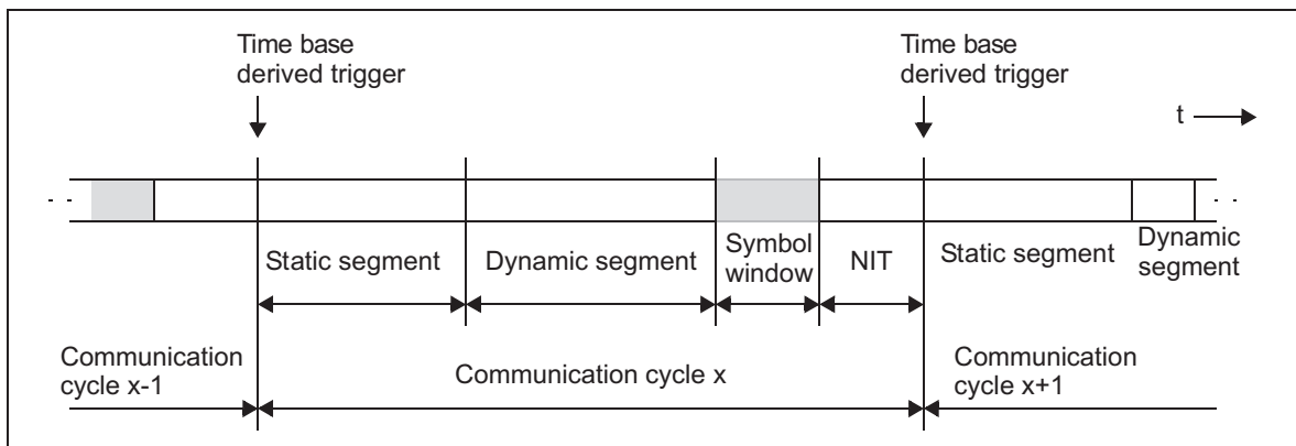
Figure 23-12. Structure of Communication Cycle
