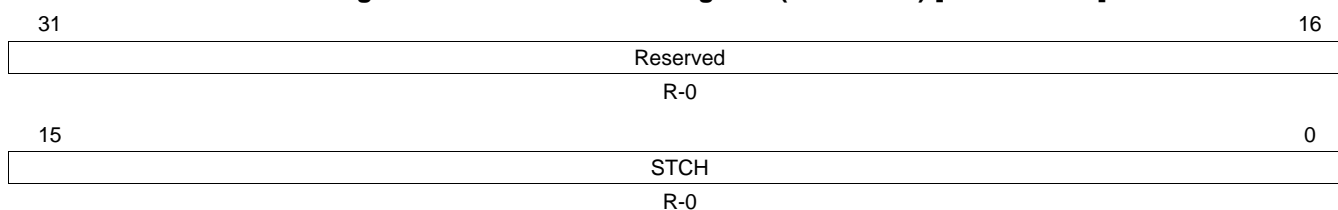
Figure 16-20. DMA Status Register (DMASTAT) [offset = 0Ch]
