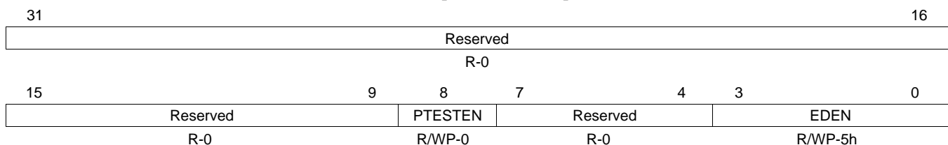
Figure 25-67. Multi-buffer RAM Uncorrectable Parity Error Control Register (UERRCTRL) [offset = 120h]
