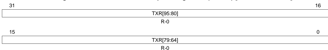
Figure 23-162. Transmission Request Register 3 (TXRQ3) [offset_CC = 328h]
