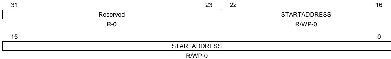
Figure 18-7. POM Program Region Start Register x (POMPROGSTARTx) [address = FFA04200h, FFA04210h, ..., FFA043F0h]
