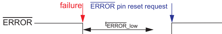
Figure 12-6. \overline{\text{ERROR}} Pin Timing - Example 3
