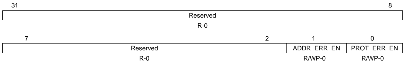
Figure 4-10. ERR_ENABLE_REG: Error Signaling Enable Register (Address = FFFF8AE8h)
