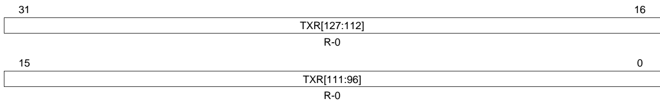
Figure 23-161. Transmission Request Register 4 (TXRQ4) [offset_CC = 32Ch]
