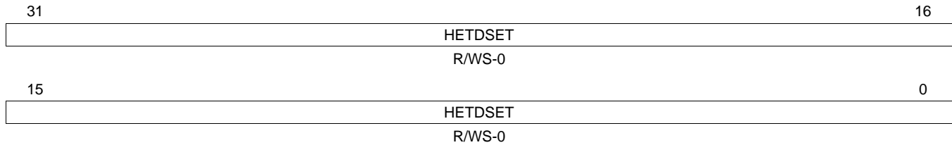
Figure 20-55. N2HET Data Set Register (HETDSET)
