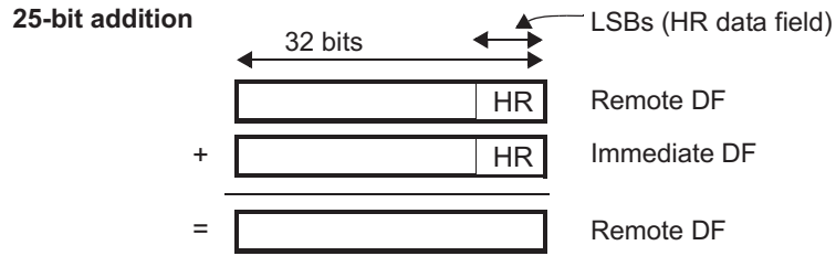
Figure 20-78. ADCNST Operation if Remote Data Field [31:7] Is Zero
