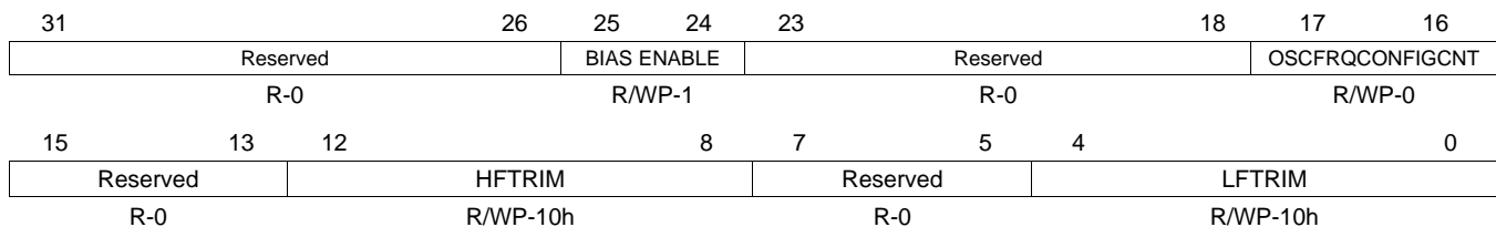
Figure 10-14. LPO/Clock Monitor Control Register (LPOMONCTL) [offset = 88h]
