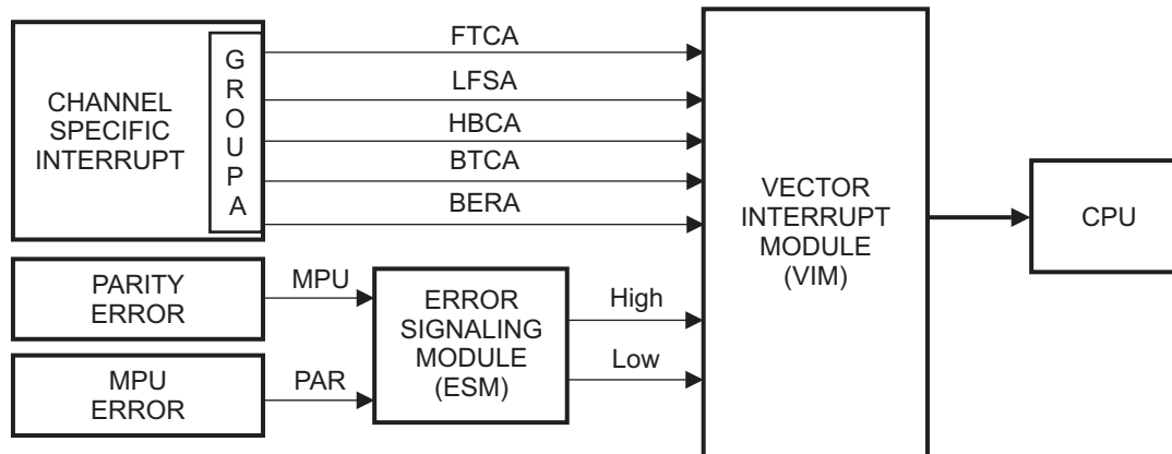
Figure 16-14. DMA Interrupts
