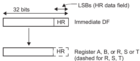
Figure 20-115. MOV32 Move Operation for IMTOREG (Case 00)
