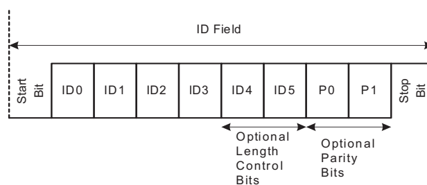
Figure 26-16. ID Field
