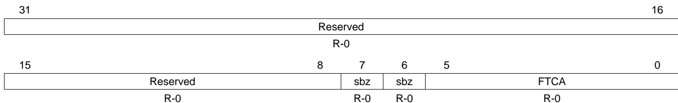
Figure 16-54. FTCA Interrupt Channel Offset Register (FTCAOFFSET) [offset = 14Ch]
