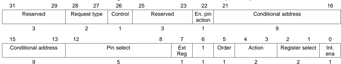
Figure 20-110. MCMP Control Field (C31:C0)
