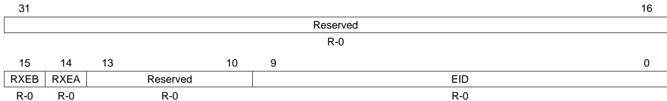
Figure 23-150. Even Sync ID Register [1..15] (ESIDn) [offset_CC = 130h-168h]
