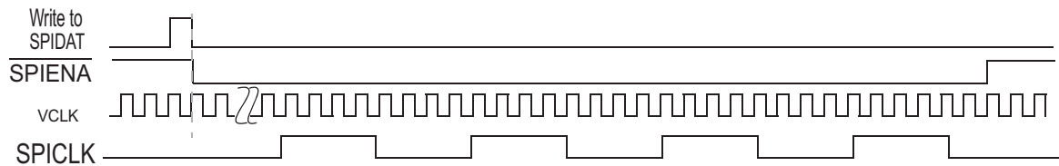
Figure 25-85. SPI/MibSPI pins during Slave mode in 4pin with \overline{\text{SPIENA}} configuration
