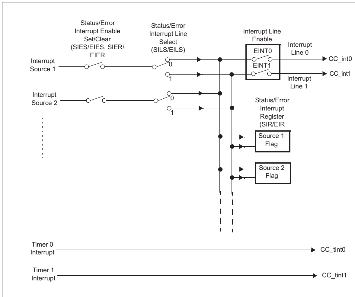
Figure 23-31. Interrupt Structure
