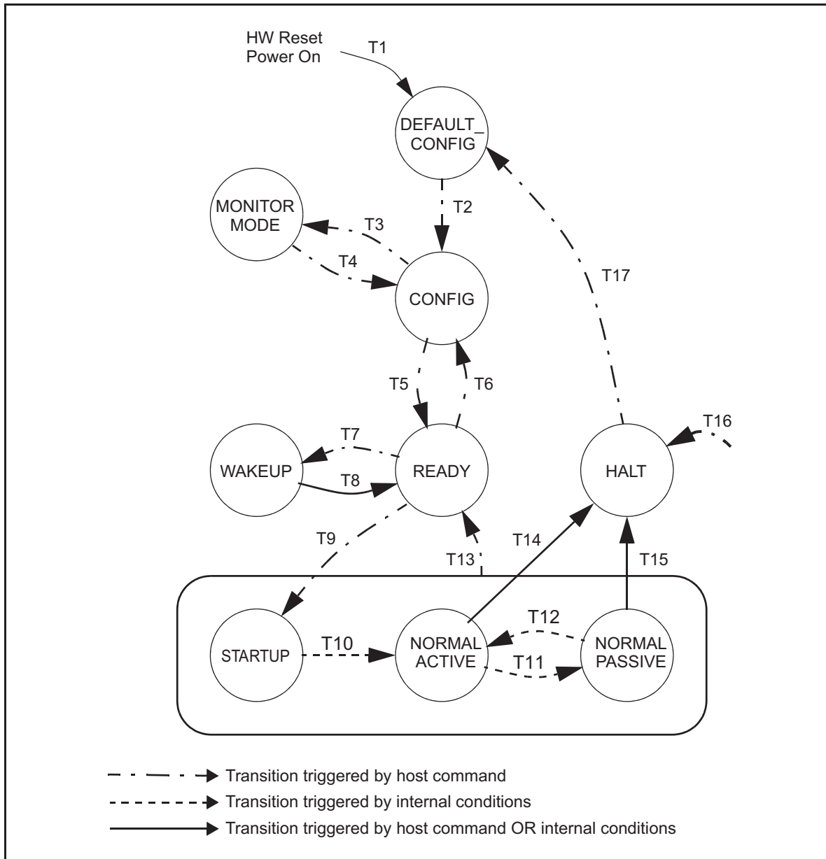
Figure 23-14. Overall State Diagram of Communication Controller
