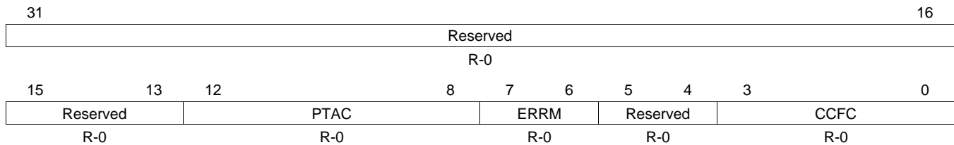
Figure 23-142. Communication Controller Error Vector Register (CCEV) [offset_CC = 104h]
