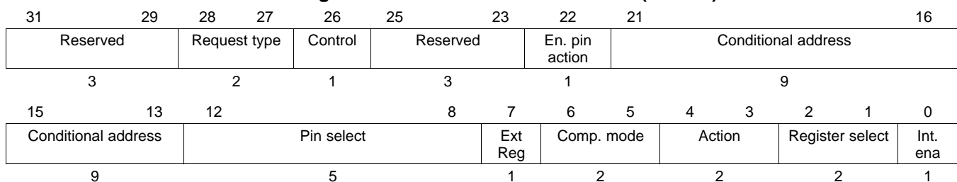
Figure 20-130. RADM64 Control Field (C31:C0)
