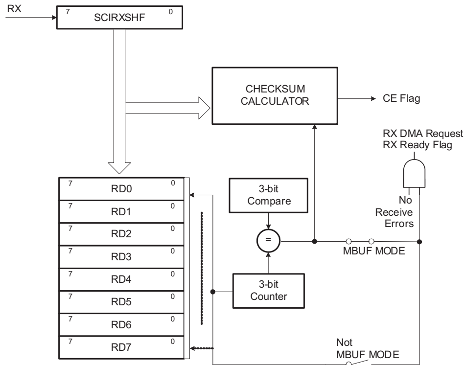
Figure 26-8. Receive Buffers
