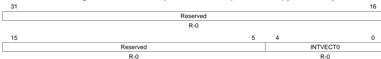
Figure 26-35. SCI Interrupt Vector Offset 0 (SCIINTVECT0) [offset = 20h]
