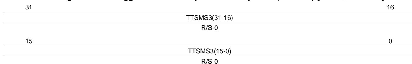
Figure 23-61. Trigger Transfer to System Memory Set 3 (TTSMS3) [offset_TU = 90h]
