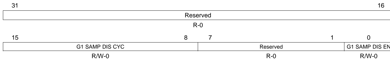
Figure 19-68. ADC Group1 Sample Cap Discharge Control Register (ADG1SAMPDISEN) [offset = 120h]
