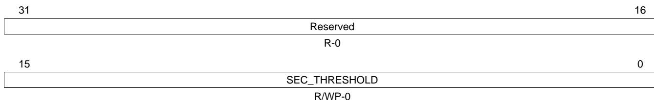
Figure 5-5. Flash Error Correction and Correction Control Register 2 (FEDACCTRL2) (offset = FFF8 700Ch)
