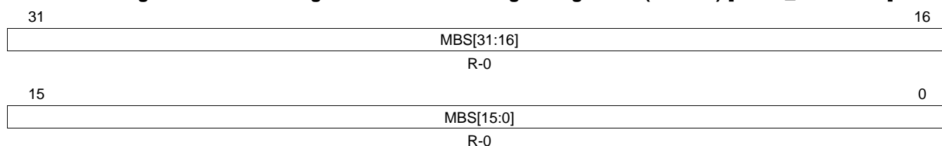
Figure 23-172. Message Buffer Status Changed Register 1 (MBSC1) [offset_CC = 340h]
