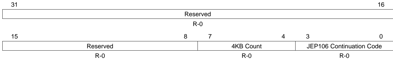
Figure 18-18. POM Peripheral ID 4 Register (POMPERIPHERALID4) [address = FFA04FD0h]
