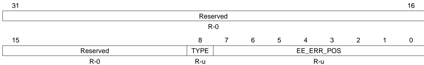
Figure 5-42. EEPROM Emulation Correctable Error Position Register (EE_COR_ERR_POS) (offset = FFF8 7318h)
