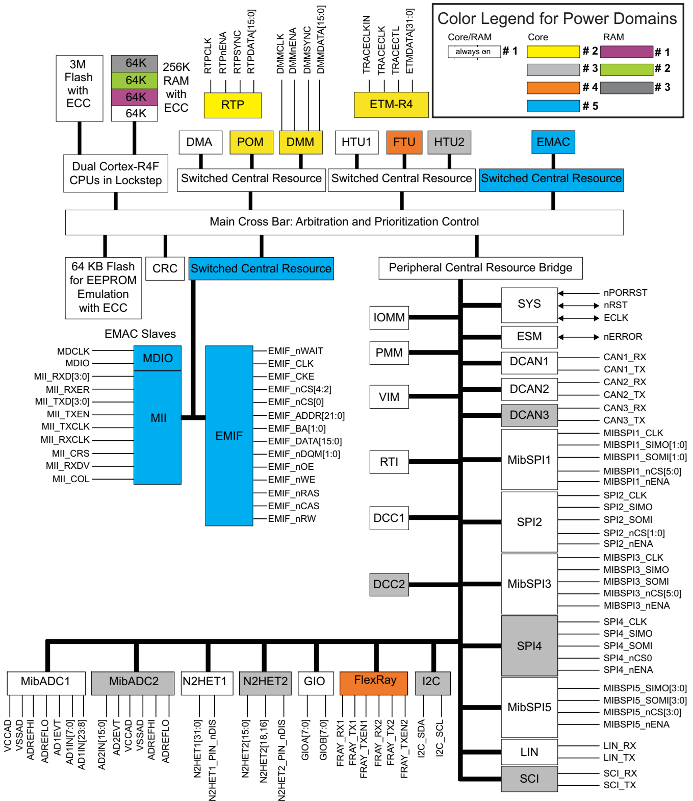
Figure 3-2 shows the core and memory power domains implemented on the microcontroller.
