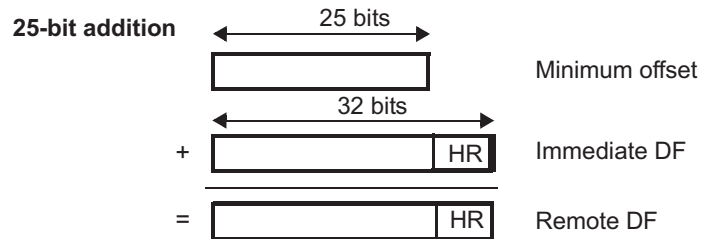
Figure 20-78. ADCNST Operation if Remote Data Field [31:7] Is Zero
