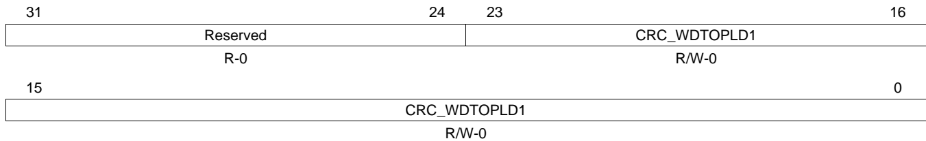
Figure 14-20. CRC Channel 1 Watchdog Timeout Preload Register A (CRC_WDTPLD1) [offset = 4Ch]
