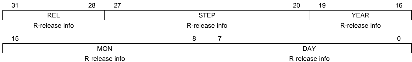
Figure 23-173. Core Release Register (CREL) [offset_CC = 3F0h]
