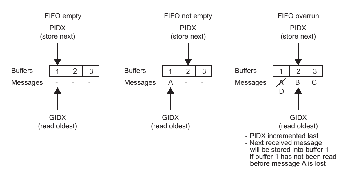
Figure 23-18. FIFO Status: Empty, Not Empty, and Overrun
