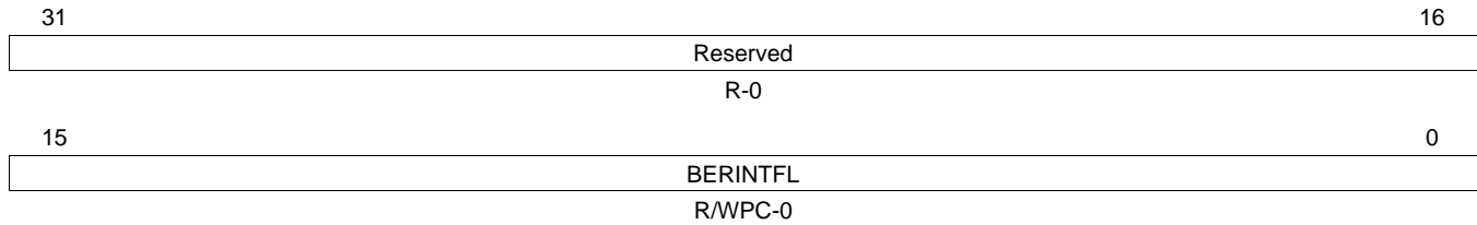
Figure 21-30. BER Interrupt Flag Register (HTU BERINTFL) [offset = 48h]
