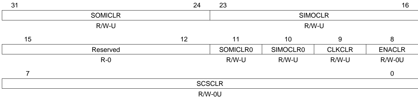
Figure 25-36. SPI Pin Control Register 5 (SPIPC5) [offset = 28h]
