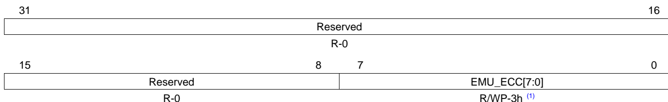
Figure 5-26. EEPROM Emulation ECC Register (FEMU_ECC) (offset = FFF8 7060h)
