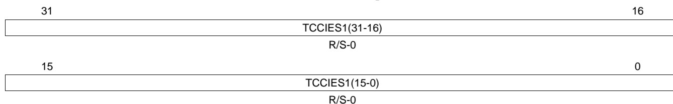
Figure 23-97. Transfer to Communication Controller Interrupt Enable Set 1 (TCCIES1) [offset_TU = 120h]
