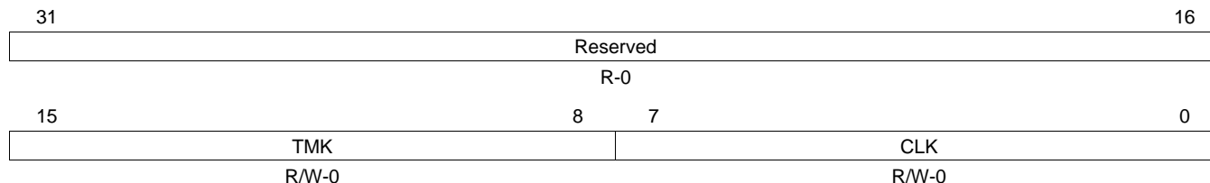
Figure 23-111. Lock Register (LCK) [offset_CC = 1Ch]
