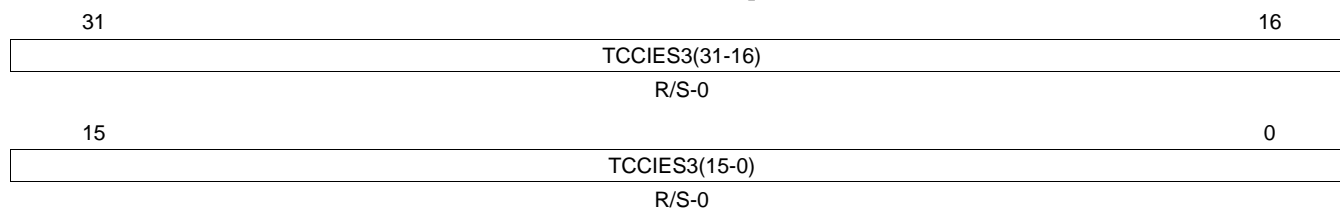
Figure 23-101. Transfer to Communication Controller Interrupt Enable Set 3 (TCCIES3) [offset_TU = 130h]
