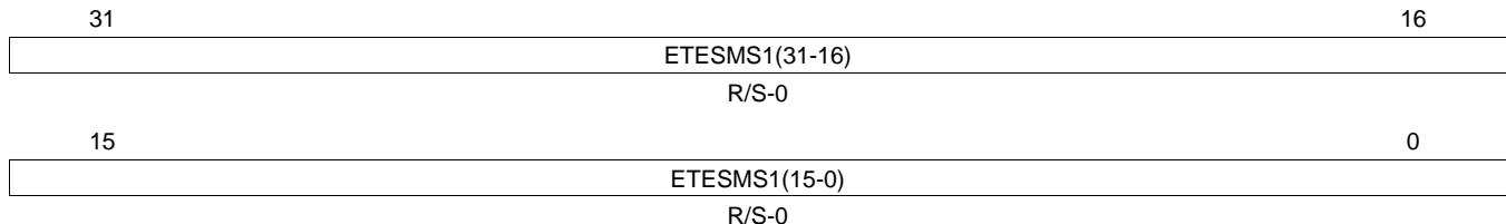
Figure 23-73. Enable Transfer on Event to System Memory Set 1 (ETESMS1) [offset_TU = C0h]
