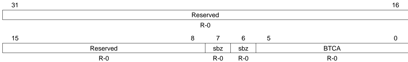
Figure 16-57. BTCA Interrupt Channel Offset Register (BTCAOFFSET) [offset = 158h]
