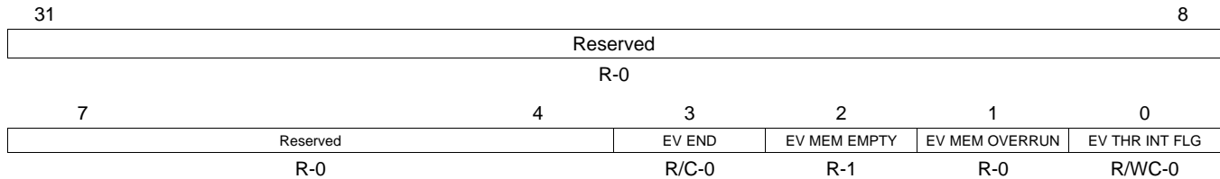
Figure 19-30. ADC Event Group Interrupt Flag Register (ADEVINTFLG) [offset = 34h]
