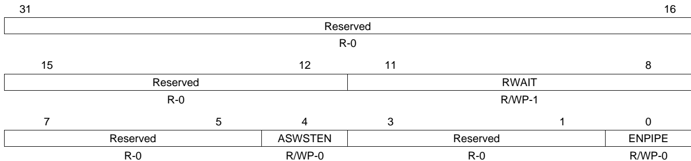
Figure 5-3. Flash Option Control Register (FRDCNTL) (offset = FFF8 7000h)
