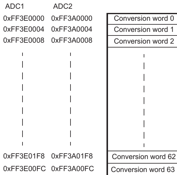
Figure 19-6. ADC Memory Mapping
