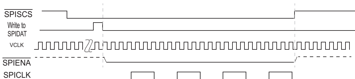
Figure 25-87. SPI/MibSPI pins during Slave mode in 5pin configuration - (Single/Multi Slave).
