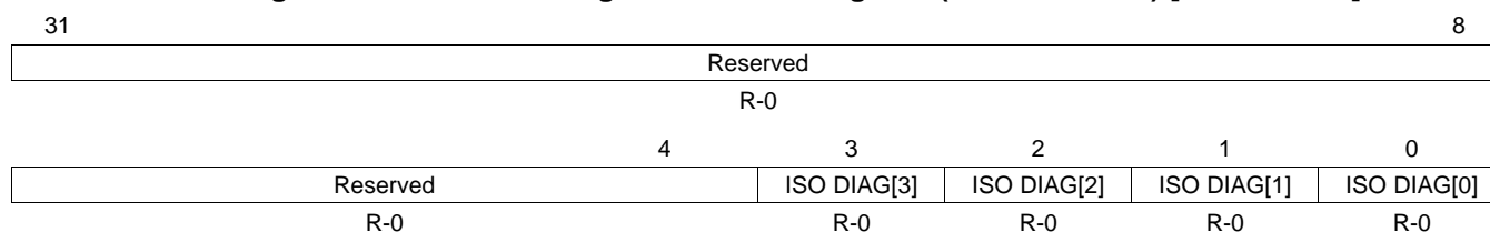
Figure 3-22. Isolation Diagnostic Status Register (ISODIAGSTAT) [offset = C0h]
