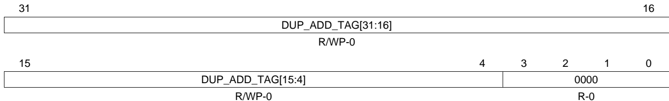
Figure 5-13. Duplicate Address Tag Register (FDUP_ADD_TAG) (offset = FFF8 702Ch)
