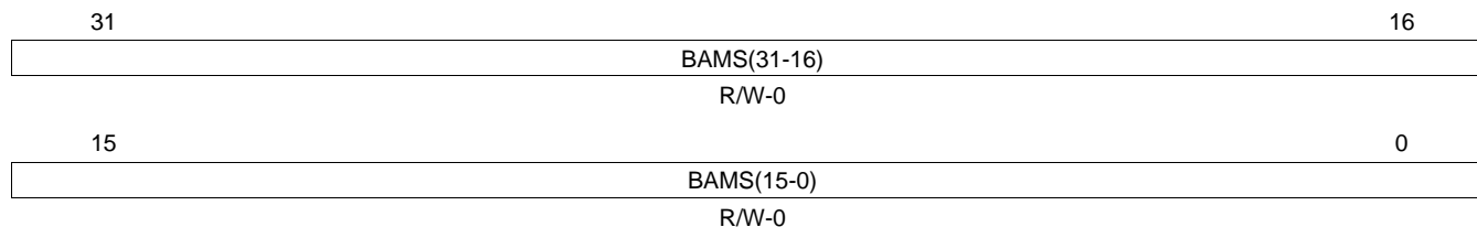
Figure 23-41. Base Address of Mirrored Status (BAMS) [offset_TU = 2Ch]
