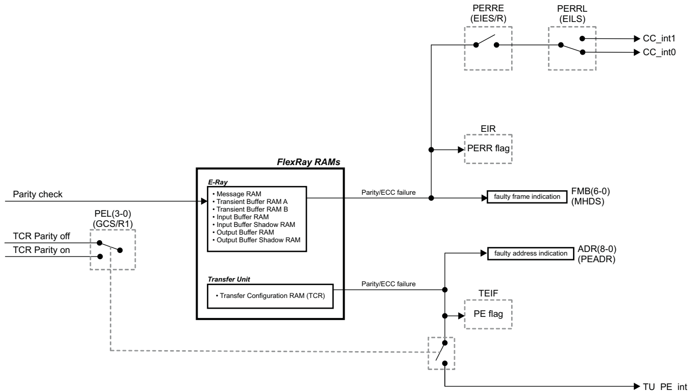
Figure 23-28. Parity Structure
