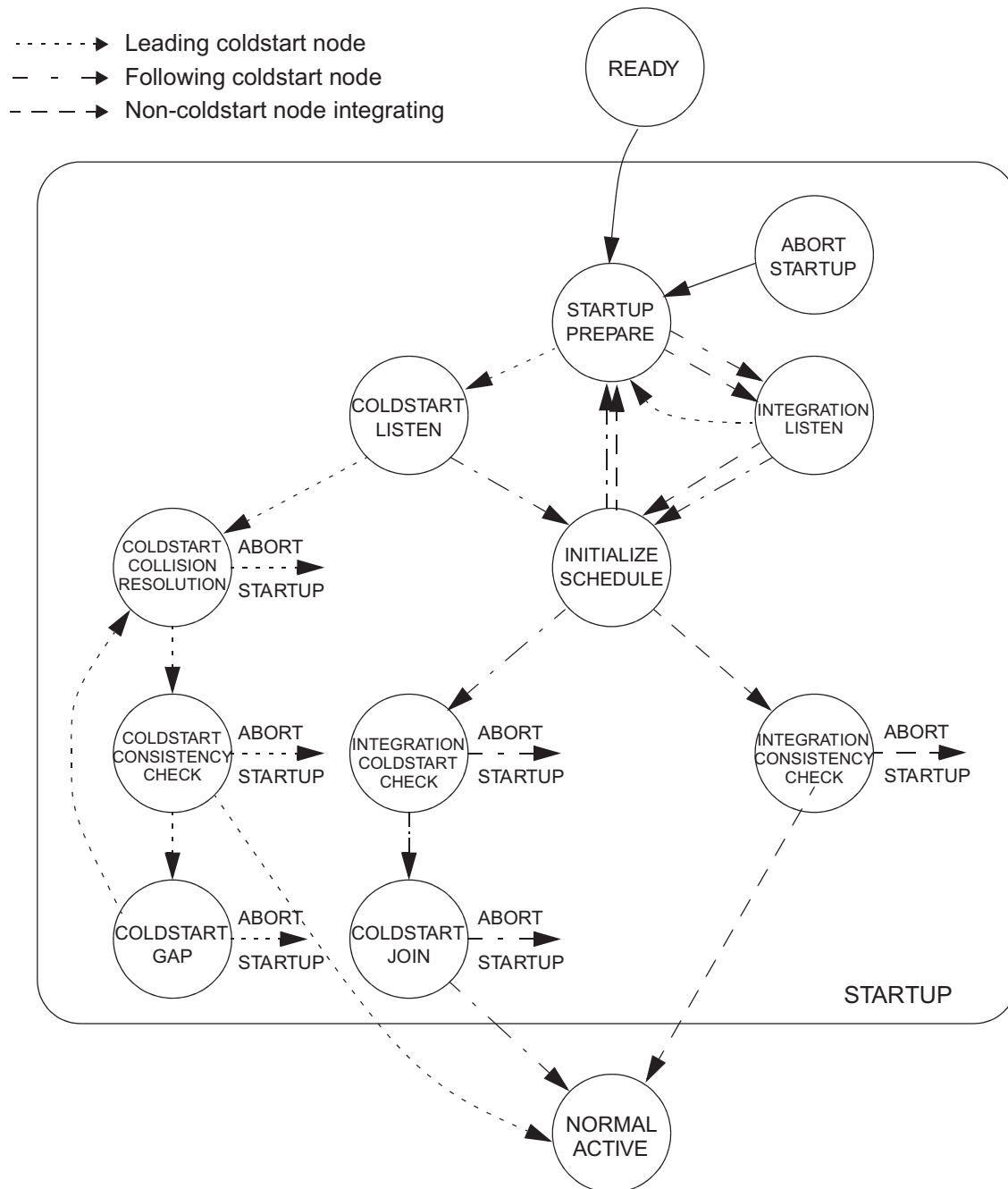
Figure 23-17. State Diagram Time-Triggered Startup
