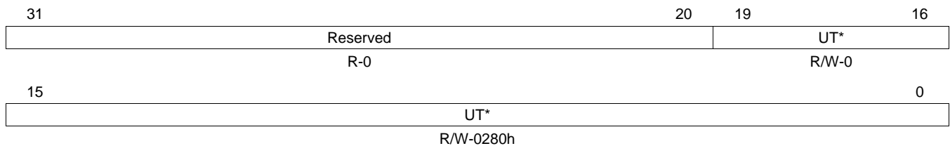
Figure 23-130. GTU Configuration Register 1 (GTUC1) [offset_CC = A0h]
