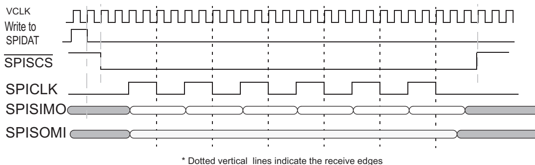
Figure 25-81. SPI/MibSPI pins during Master mode 4-pin with \overline{\text{SPISCS}} configuration.
