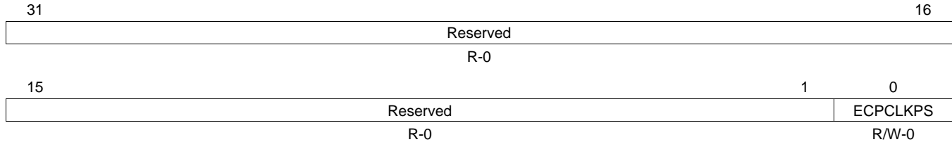
Figure 2-14. SYS Pin Control Register 9 (SYSPC9) [offset = 20h]
