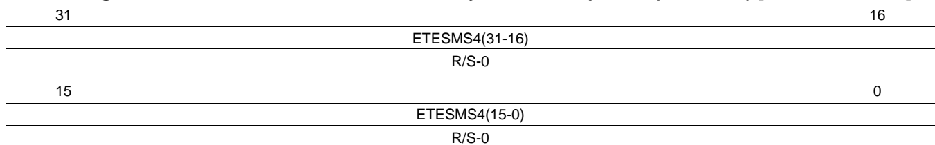
Figure 23-79. Enable Transfer on Event to System Memory Set 4 (ETESMS4) [offset_TU = D8h]
