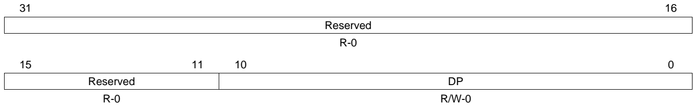
Figure 23-178. Write Header Section Register 3 (WRHS3) [offset_CC = 508h]
