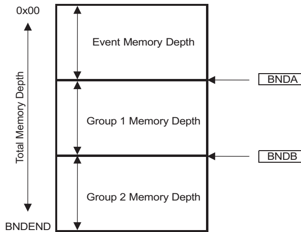
Figure 19-3. FIFO Implementation
