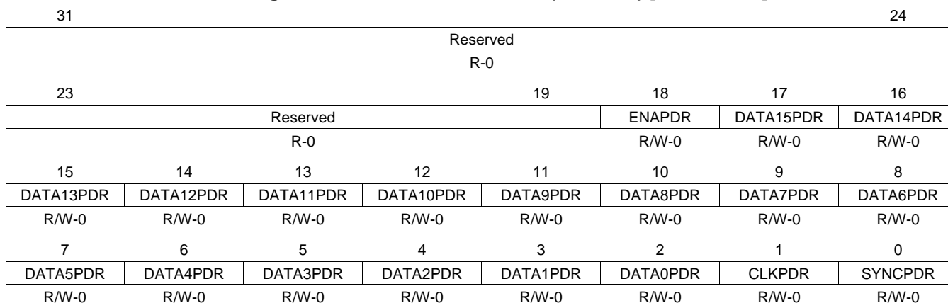
Figure 30-28. DMM Pin Control 6 (DMMP6) [offset = 84h]
