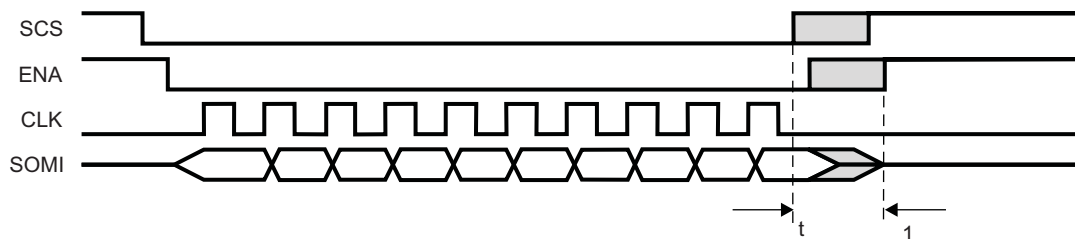
Figure 25-47. Transmit-Data-Finished-to-ENA-Inactive-Timeout
