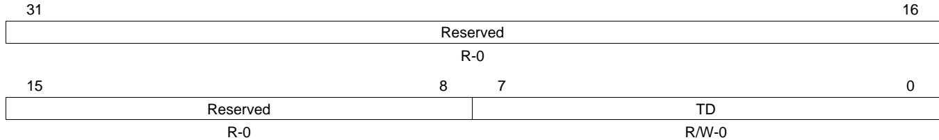
Figure 26-41. Transmit Data Buffer Register (SCITD) [offset = 38h]
