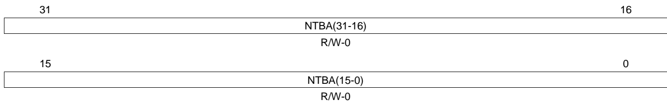
Figure 23-40. Next Transfer Base Address (NTBA) [offset_TU = 28h]
