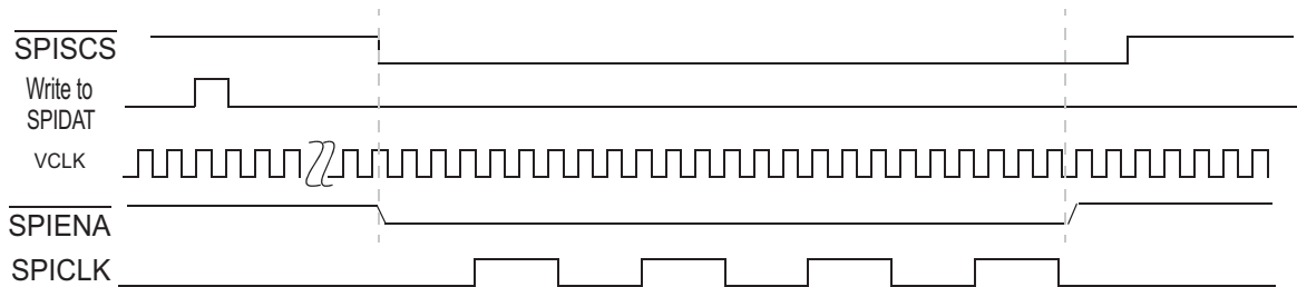
Figure 25-86. SPI/MibSPI pins during Slave mode in 5pin configuration - (Single Slave).
