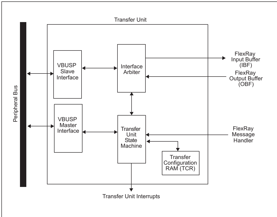
Figure 23-3. Transfer Unit
