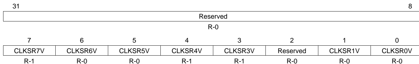
Figure 2-24. Clock Source Valid Status Register (CSVSTAT) [offset = 54h]
