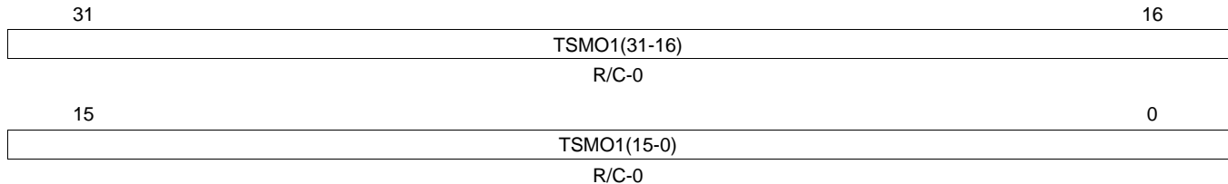
Figure 23-44. Transfer to System Memory Occurred 1 (TSMO1) [offset_TU = 40h]
