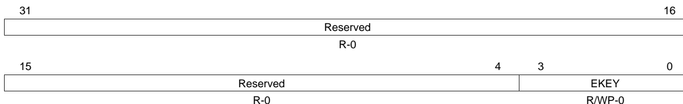
Figure 12-25. ESM Error Key Register (ESMEKR) [offset = FFFF F538h]
