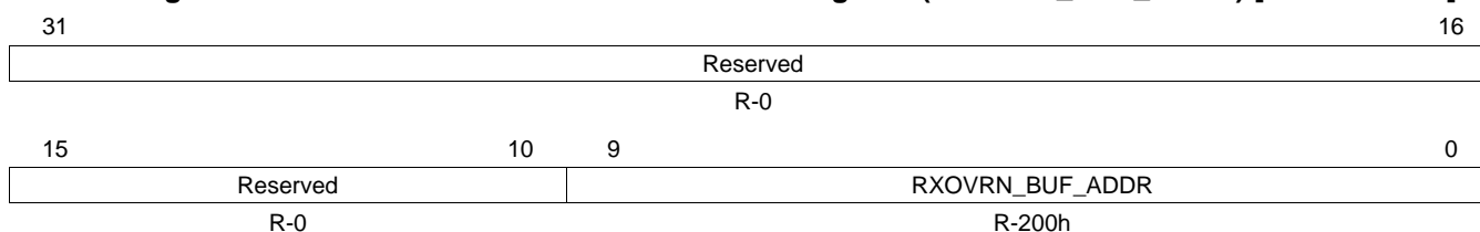
Figure 25-71. RXRAM Overrun Buffer Address Register (RXOVRN_BUF_ADDR) [offset = 130h]
