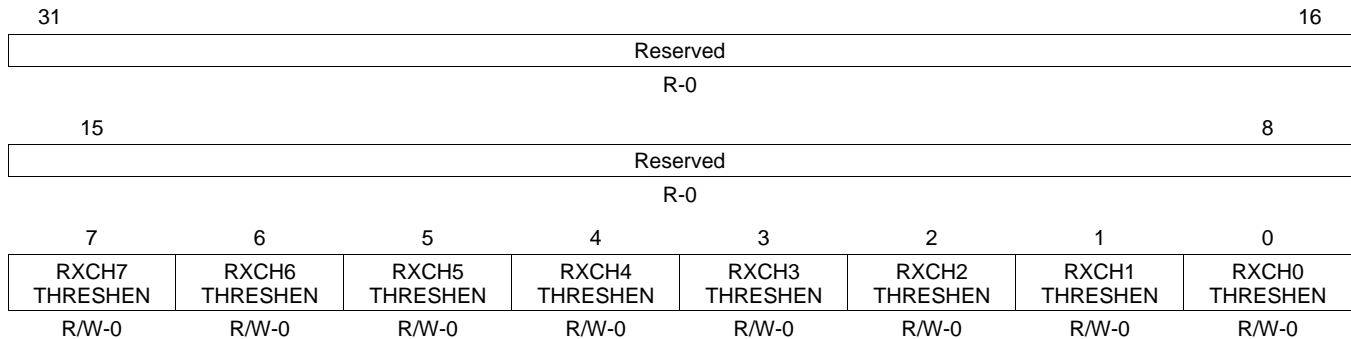
Figure 29-15. EMAC Control Module Receive Threshold Interrupt Enable Register (C0RXTHRESHEN)
