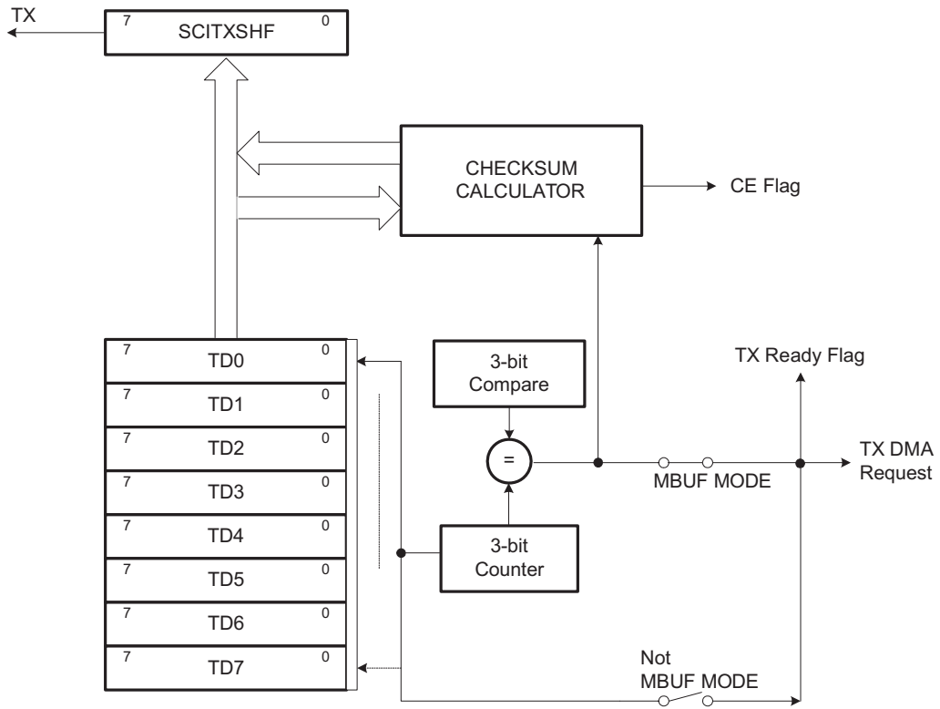
Figure 26-9. Transmit Buffers
