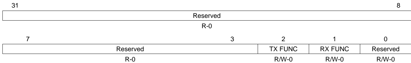
Figure 27-28. SCI Pin I/O Control Register 6 (SCIPIO6) [offset = 54h]
