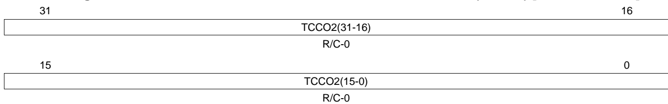
Figure 23-49. Transfer to Communication Controller Occurred 2 (TCCO2) [offset_TU = 54h]
