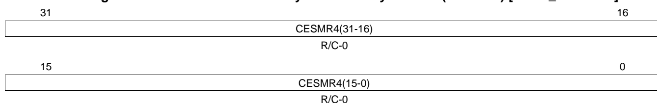
Figure 23-88. Clear on Event to System Memory Reset 4 (CESMR4) [offset_TU = FCh]
