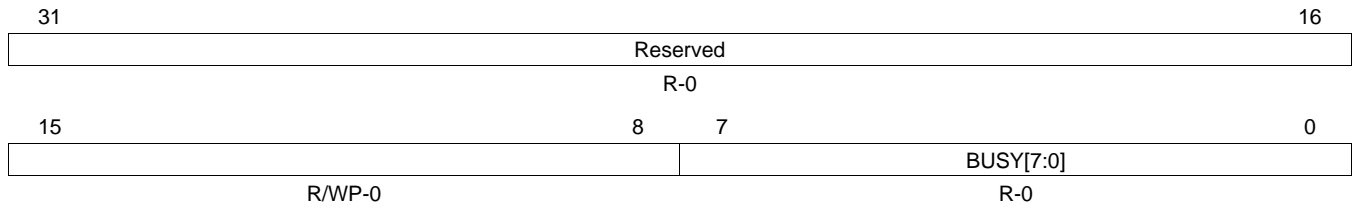
Figure 5-16. Flash Bank Busy Register (FBBUSY) (offset = FFF8 7038h)
