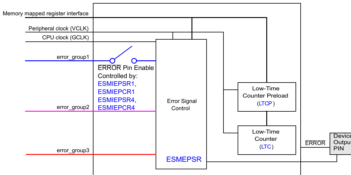
Figure 12-3. ERROR Pin Response Handling
