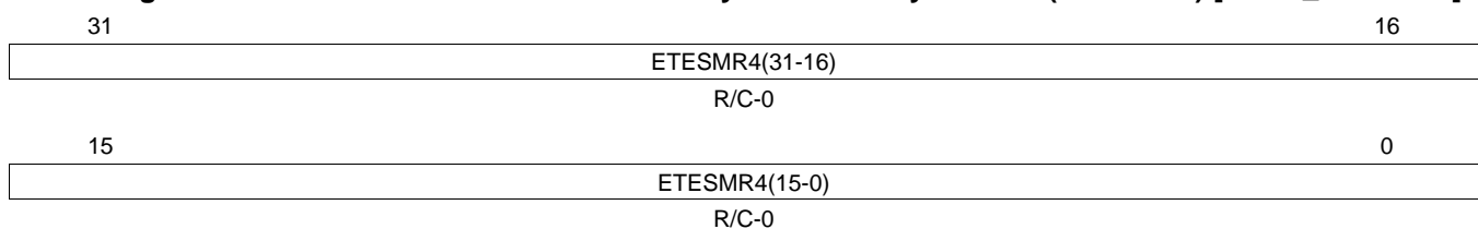
Figure 23-80. Enable Transfer on Event to System Memory Reset 4 (ETESMR4) [offset_TU = DCh]
