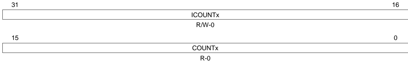
Figure 25-65. DMAxCOUNT Register (ICOUNT) [offset = F8h-114h]
