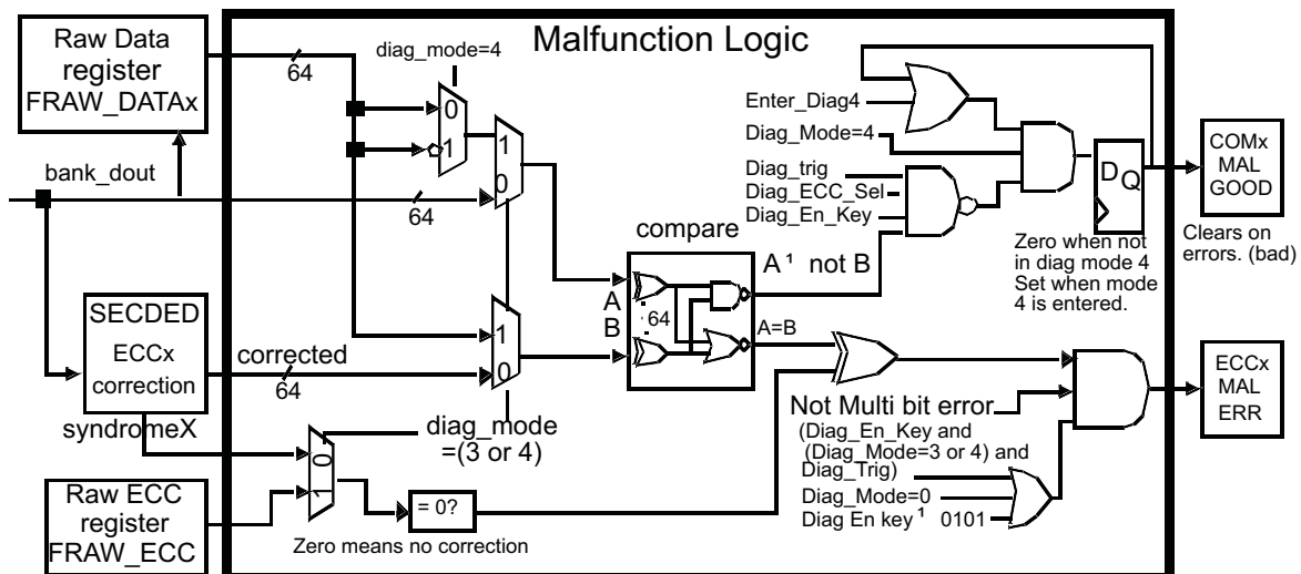
Figure 5-2. ECC Malfunction Test Logic
