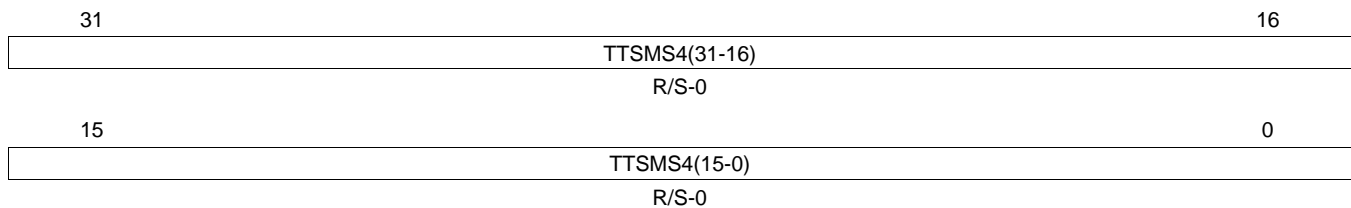
Figure 23-63. Trigger Transfer to System Memory Set 4 (TTSMS4) [offset_TU = 98h]
