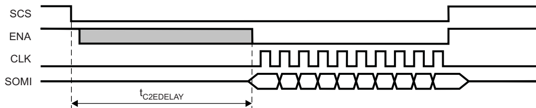
Figure 25-48. Chip-Select-Active-to-ENA-Signal-Active-Timeout
