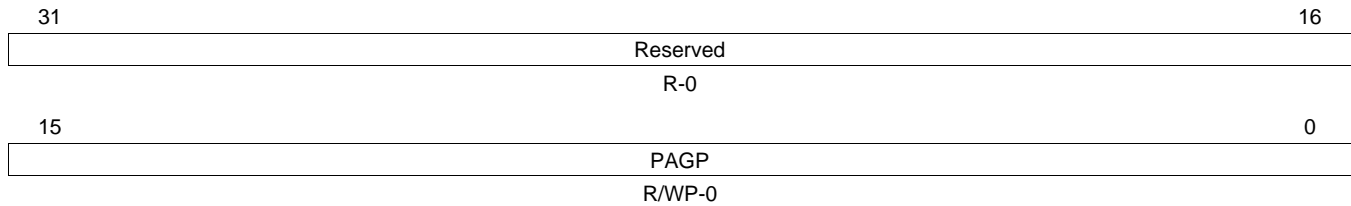
Figure 5-21. Flash Pump Access Control Register 2 (FPAC2) (offset = FFF8 704Ch)
