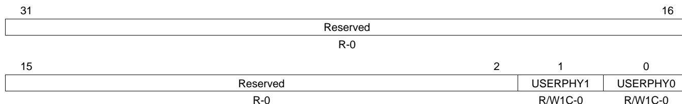
Figure 29-29. MDIO Link Status Change Interrupt (Unmasked) Register (LINKINTRAW)
