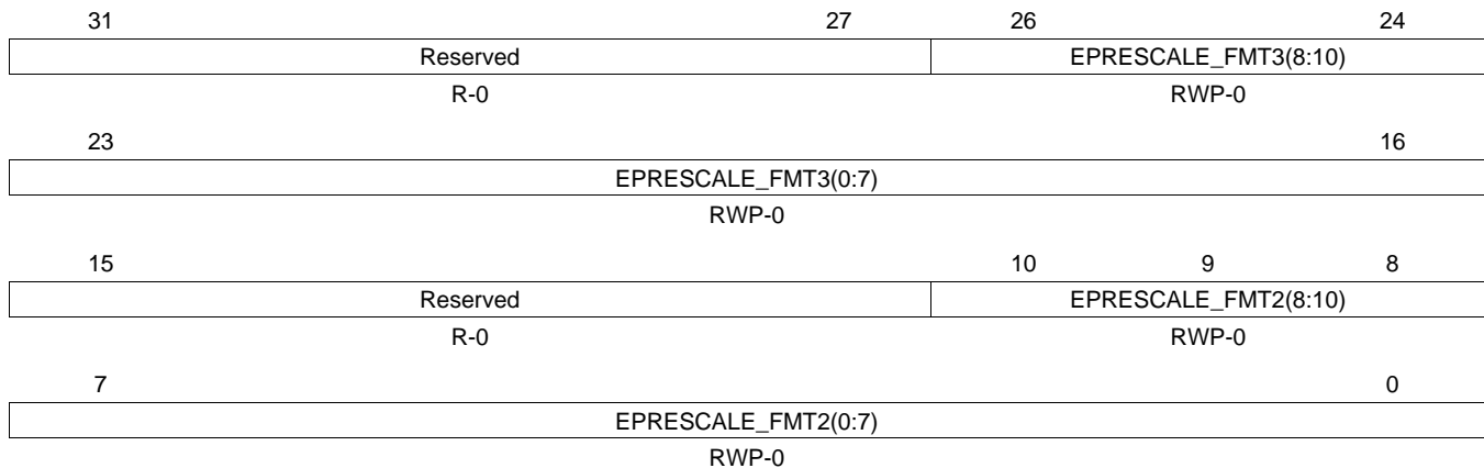
Figure 25-74. SPI Extended Prescale Register 2 (EXTENDED_PRESCALE2 for SPIFMT2 and SPIFMT3) [offset = 13Ch]
