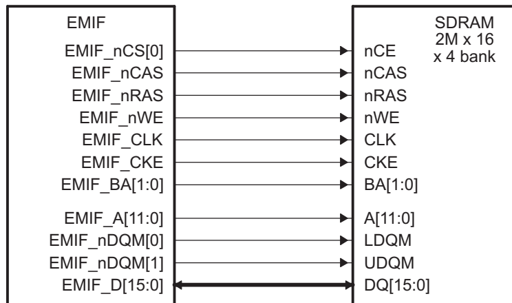
Figure 17-3. EMIF to 2M x 16 x 4 bank SDRAM Interface
