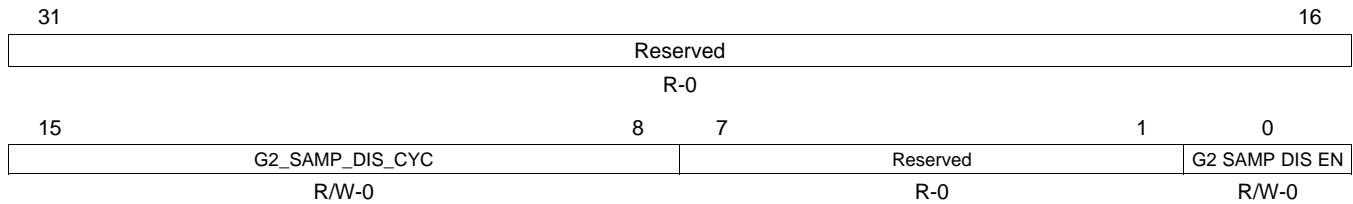
Figure 19-69. ADC Group2 Sample Cap Discharge Control Register (ADG2SAMPDISEN) [offset = 124h]
