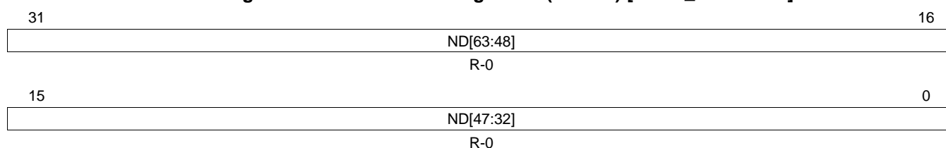
Figure 23-167. New Data Register 2 (NDAT2) [offset_CC = 334h]
