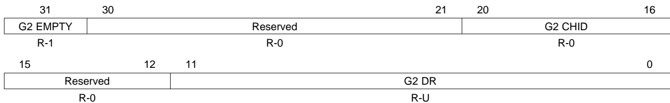
Figure 19-57. 12-bit ADC Group2 Results FIFO Register (ADG2BUFFER) [offset = D0h - EFh]
