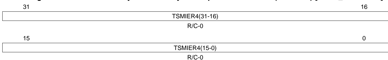
Figure 23-96. Transfer to System Memory Interrupt Enable Reset 4 (TSMIER4) [offset_TU = 11Ch]
