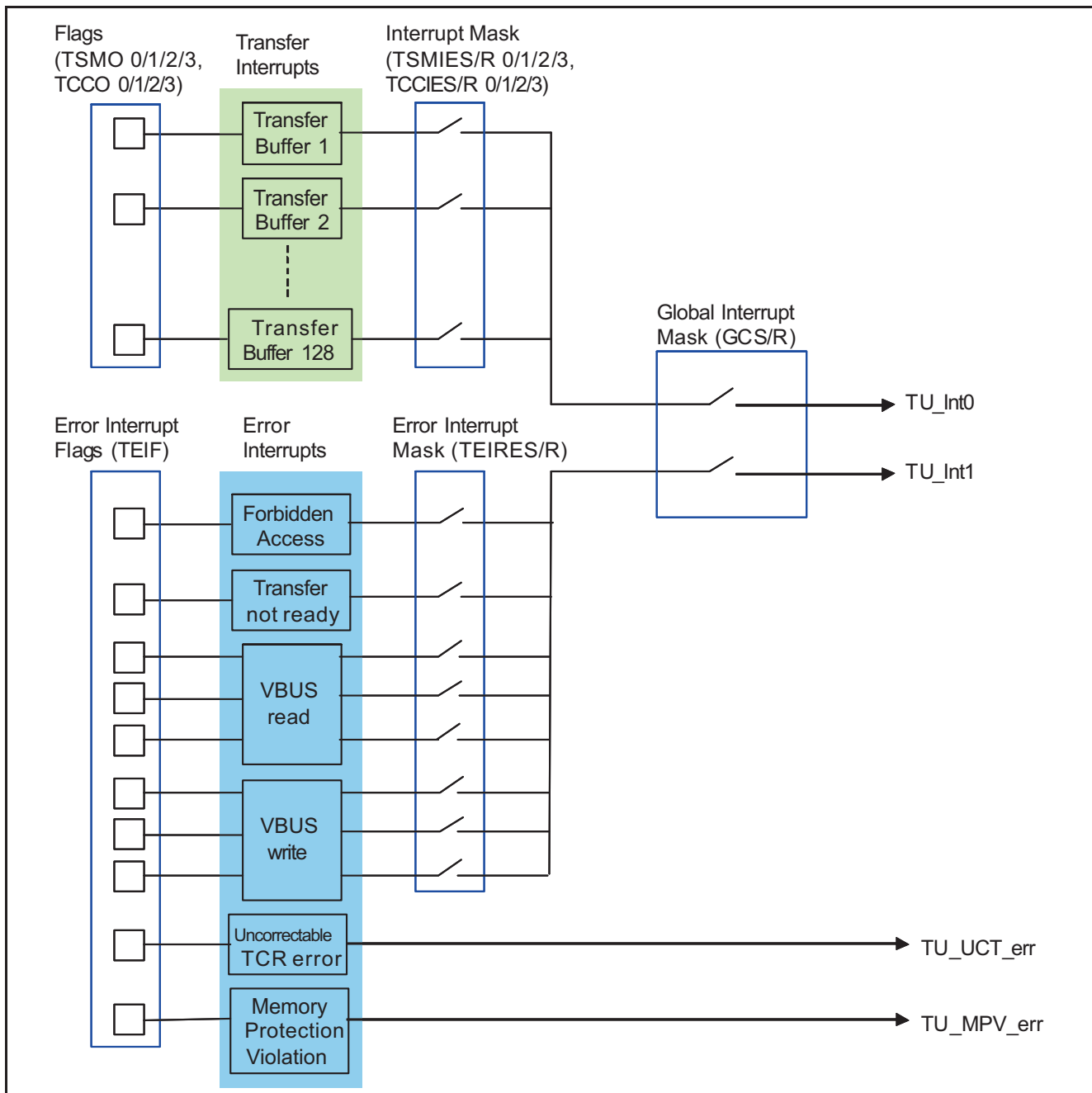
Figure 23-30. Transfer Unit Interrupt Structure
