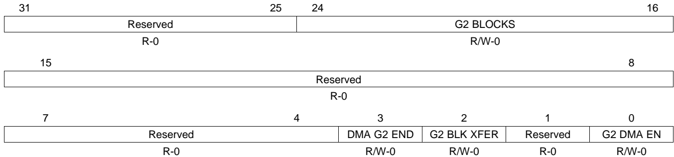
Figure 19-38. ADC Group2 DMA Control Register (ADG2DMACR) [offset = 54h]
