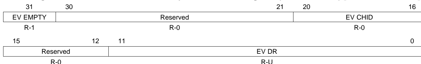
Figure 19-53. 12-bit ADC Event Group Results' FIFO Register (ADEVBUFFER) [offset = 90h - AFh]
