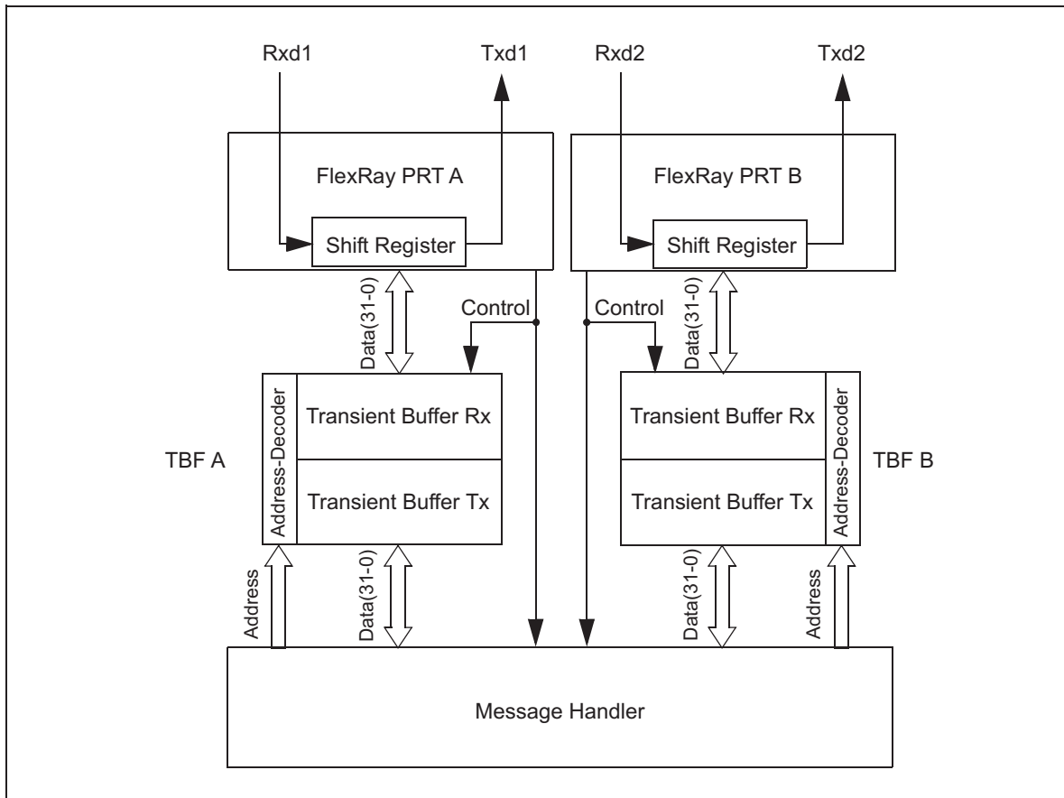
Figure 23-24. Access to Transient Buffer RAMs
