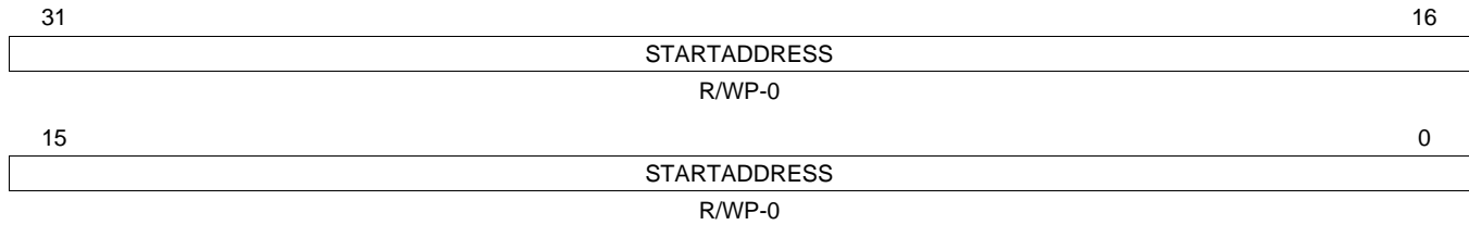
Figure 16-80. DMA Memory Protection Region 2 Start Address Register (DMAMPR2S) [offset = 1C8h]
