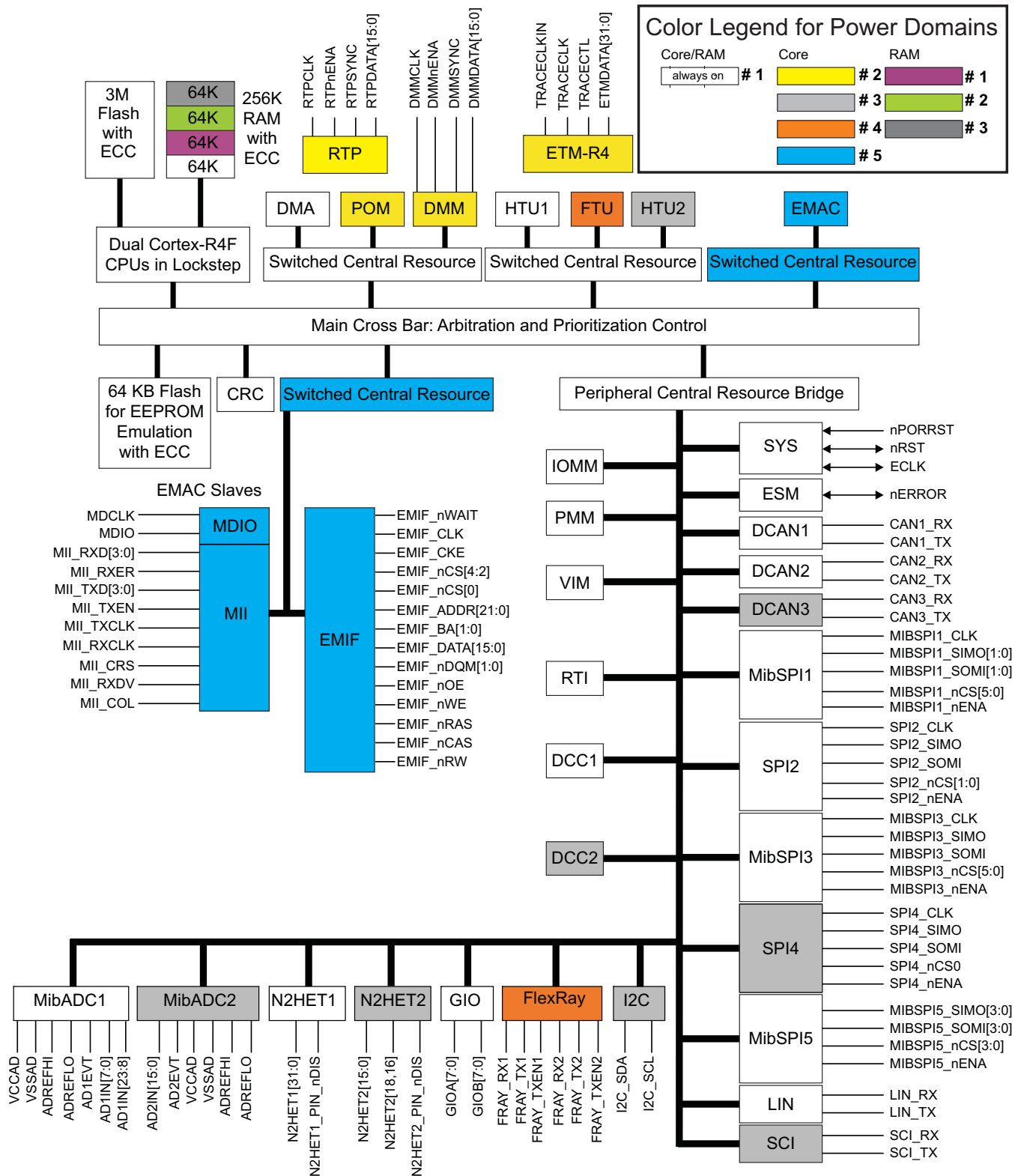
Figure 1-1. Block Diagram
