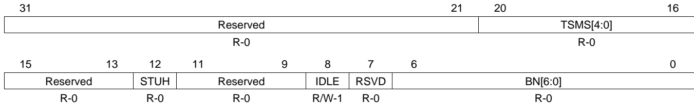
Figure 23-36. Transfer Status Current Buffer (TSCB) [offset_TU = 18h]
