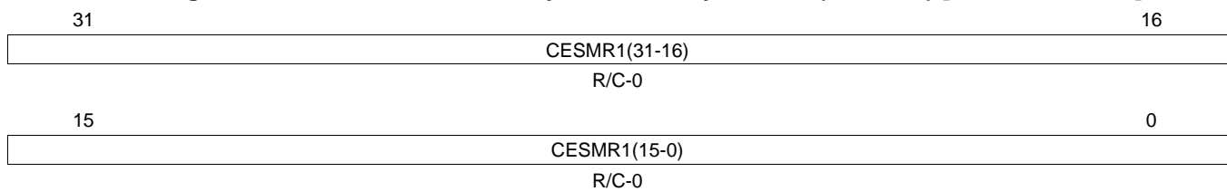
Figure 23-82. Clear on Event to System Memory Reset 1 (CESMR1) [offset_TU = E4h]
