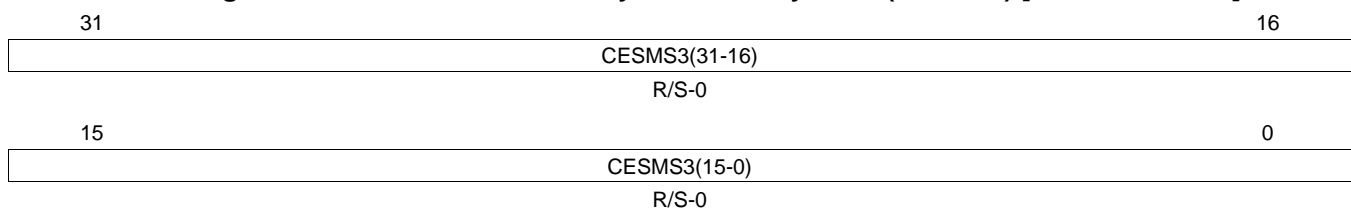
Figure 23-85. Clear on Event to System Memory Set 3 (CESMS3) [offset_TU = F0h]
