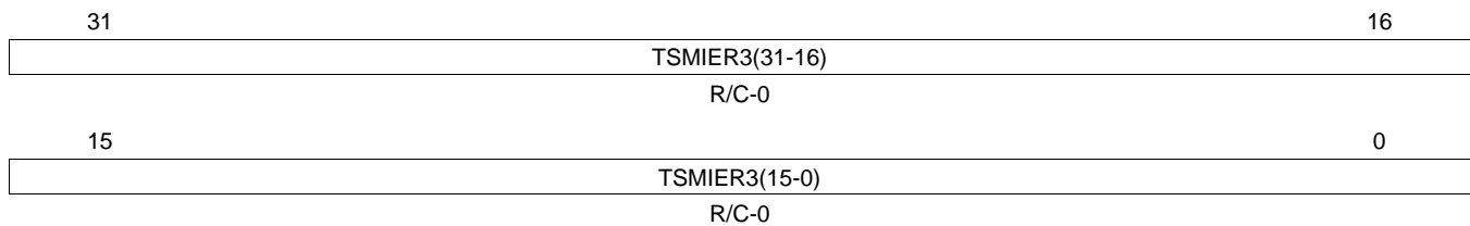
Figure 23-94. Transfer to System Memory Interrupt Enable Reset 3 (TSMIER3) [offset_TU = 114h]
