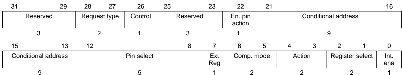
Figure 20-120. MOV64 Control Field (C31:C0)
