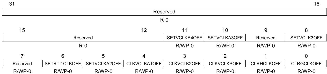
Figure 2-19. Clock Domain Disable Set Register (CDDISSET) [offset = 40h]
