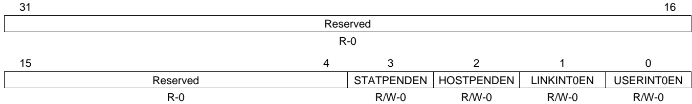
Figure 29-18. EMAC Control Module Miscellaneous Interrupt Enable Register (COMISCEN)
