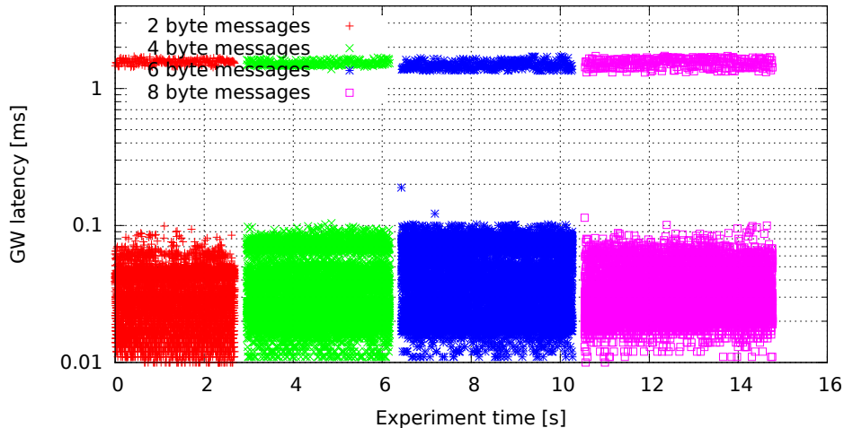
Single GW rule for all messages, no modifications (GW kernel rtems4.10-midam, Traffic oneatatime, Load eth)
