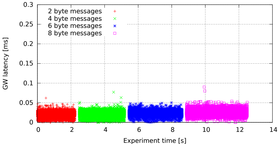
Single GW rule for all messages, no modifications, high (soft)irq task priority (GW kernel rtems4.10-midam, Traffic oneatatime, Load eth)
