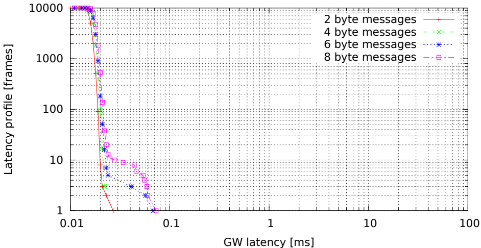
Single GW rule for all messages, no modifications, high (soft)irq task priority (GW kernel rtems4.10-midam, Traffic oneatatime, Load cpu)
