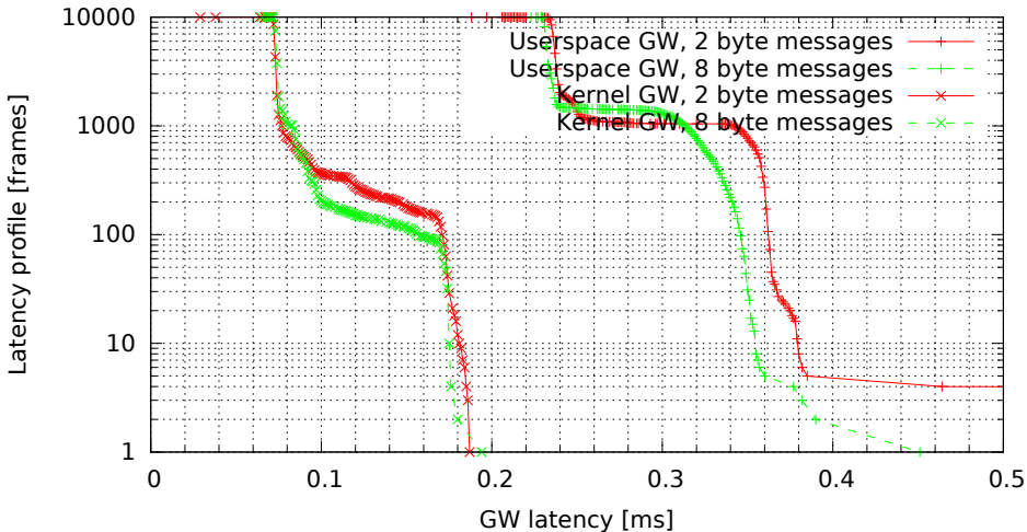
Kernel vs. userspace GW, no modifications (GW kernel 3.4.33-rt47-00004-gc58c9ae, Traffic oneatatime, Load none)
