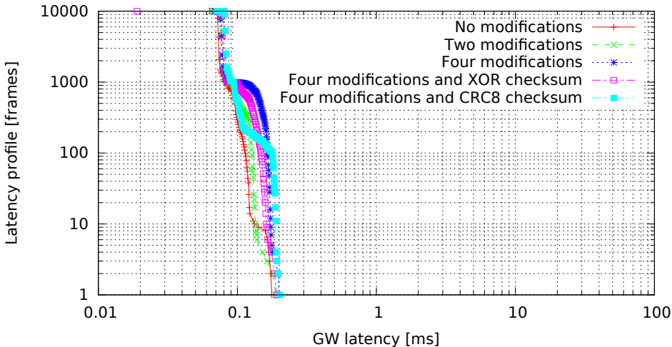
Single GW rule for all messages with modifications, 8 byte messages (GW kernel 3.4.33-rt47-00004-gc58c9ae, Traffic oneatatime, Load none)
