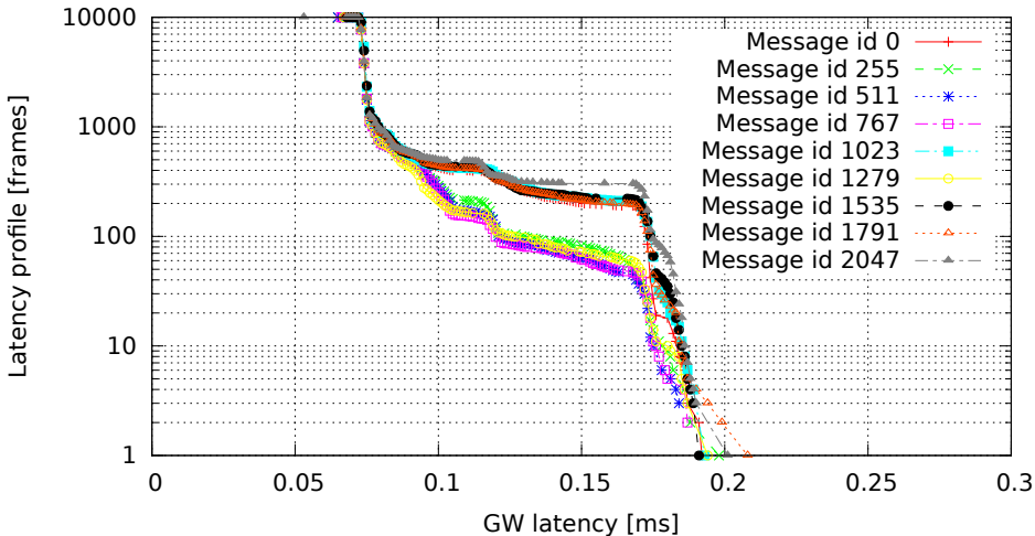
2048 GW rules (one per id, mask C00007FF), no modifications (GW kernel 3.4.33-rt47-00004-gc58c9ae, Traffic oneatatime, Load none)
