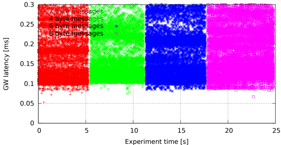
Single GW rule for all messages, no modifications (GW kernel 3.4.33-rt47-00004-gc58c9ae, Traffic oneatatime, Load eth)
