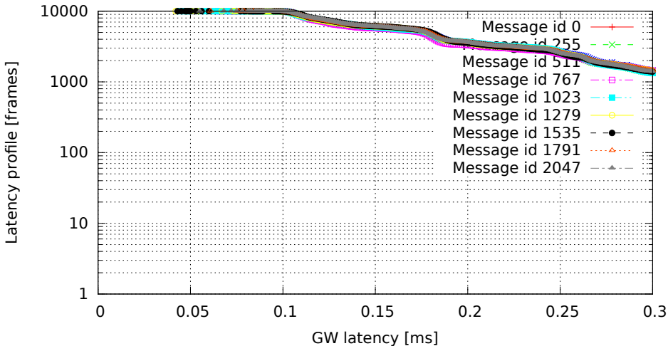
2048 GW rules (one per id, mask C00007FF), no modifications (GW kernel 3.4.33-rt47-00004-gc58c9ae, Traffic oneatatime, Load eth)
