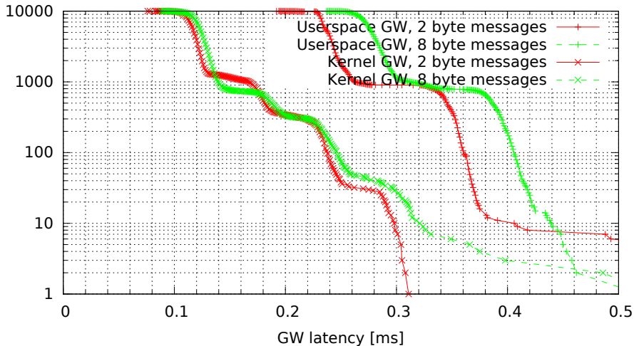
Kernel vs. userspace GW, no modifications (GW kernel 3.4.33-rt47-00004-gc58c9ae, Traffic oneatotime, Load cpu)
