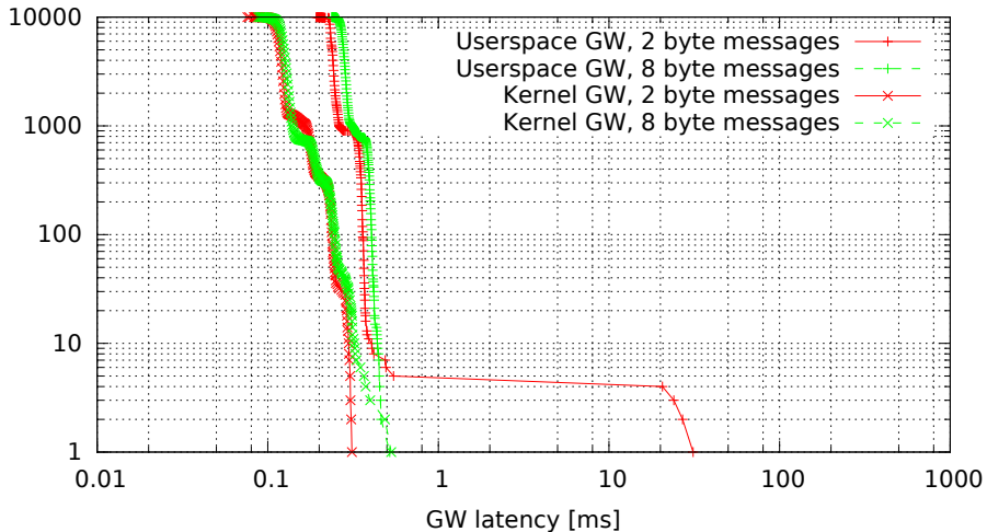
Kernel vs. userspace GW, no modifications (GW kernel 3.4.33-rt47-00004-gc58c9ae, Traffic oneatatime, Load cpu)
