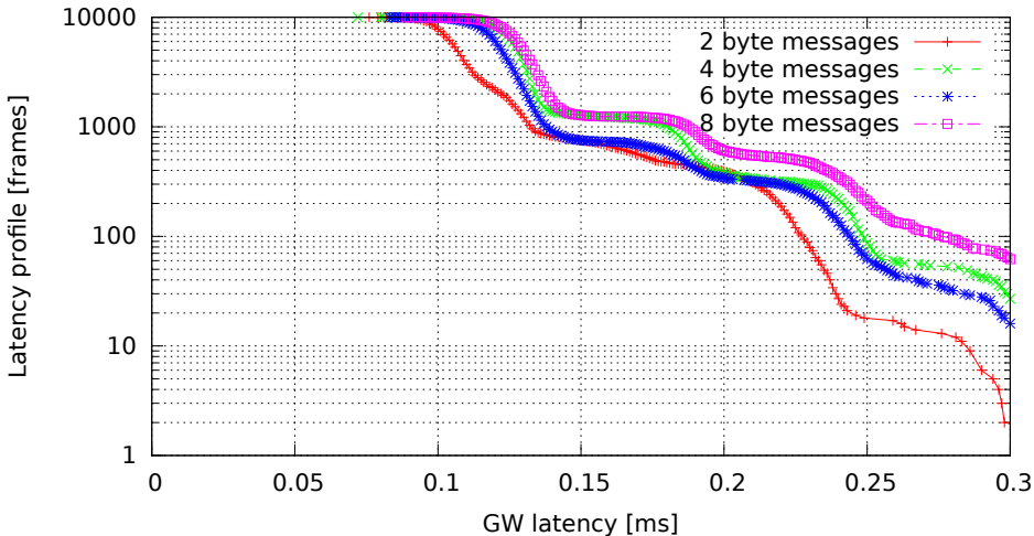
Single GW rule for all messages, no modifications, high (soft)irq task priority (GW kernel 3.4.33-rt47-00004-gc58c9ae, Traffic oneatotime, Load cpu)
