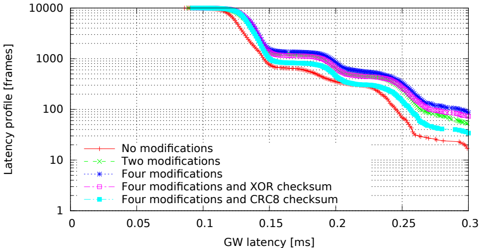
Single GW rule for all messages with modifications, 8 byte messages (GW kernel 3.4.33-rt47-00004-gc58c9ae, Traffic oneatime, Load cpu)
