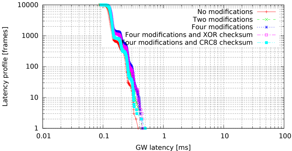
Single GW rule for all messages with modifications, 8 byte messages (GW kernel 3.4.33-rt47-00004-gc58c9ae, Traffic oneatotime, Load cpu)
