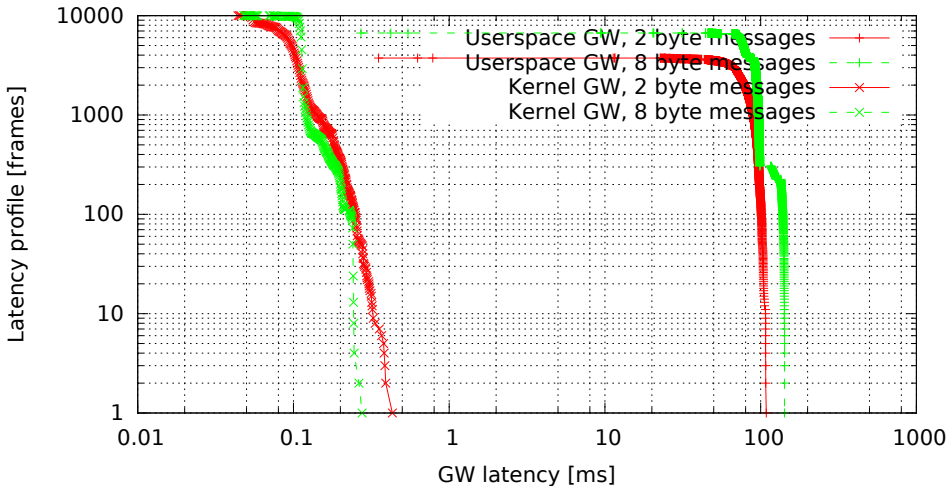
Kernel vs. userspace GW, no modifications (GW kernel 3.4.33-rt47-00004-gc58c9ae, Traffic flood, Load none)
