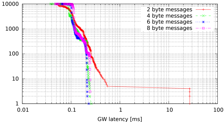
Single GW rule for all messages, no modifications, high (soft)irq task priority (GW kernel 3.4.33-rt47-00004-gc58c9ae, Traffic flood, Load none)
