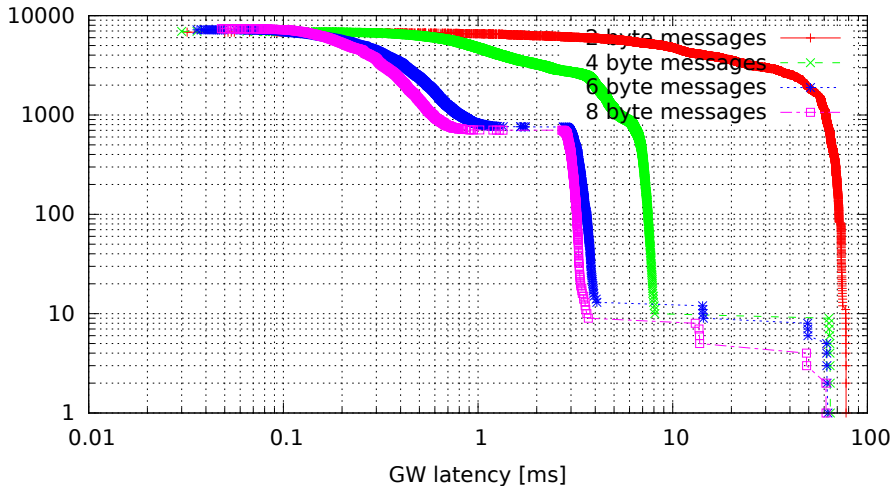
Single GW rule for all messages, no modifications (GW kernel 3.4.33-rt47-00004-gc58c9ae, Traffic flood, Load eth)
