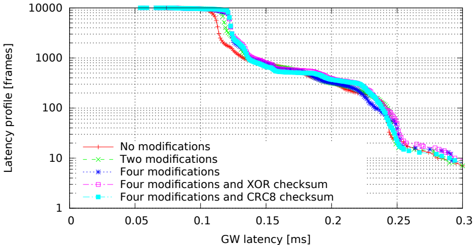
Single GW rule for all messages with modifications, 8 byte messages (GW kernel 3.4.33-rt47-00004-gc58c9ae, Traffic flood, Load cpu)
