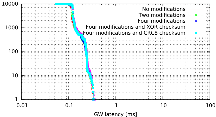
Single GW rule for all messages with modifications, 8 byte messages (GW kernel 3.4.33-rt47-00004-gc58c9ae, Traffic flood, Load cpu)
