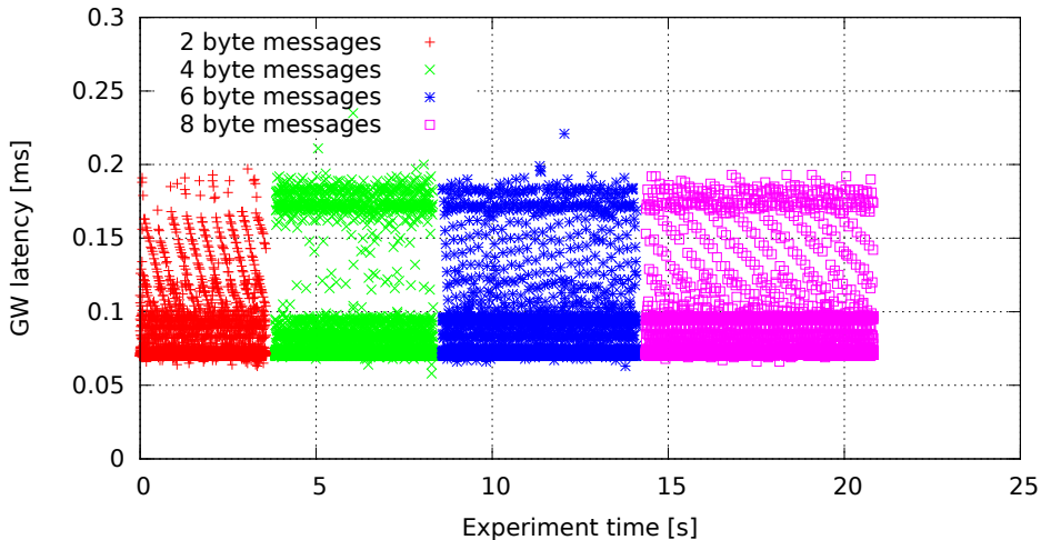
Single GW rule for all messages, no modifications, high (soft)irq task priority (GW kernel 3.4.33-rt47-00004-gc58c9ae, Traffic 50, Load none)
