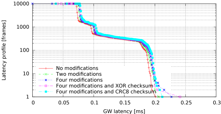
Single GW rule for all messages with modifications, 8 byte messages (GW kernel 3.4.33-rt47-00004-gc58c9ae, Traffic 50, Load none)
