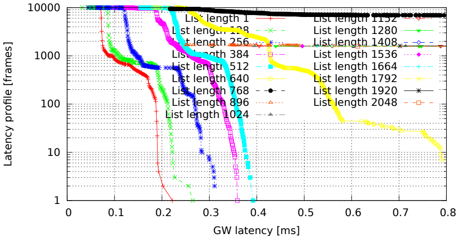
Different lengths of filter list, only the last one matches (GW kernel 3.4.33-rt47-00004-gc58c9ae, Traffic 50, Load none)
