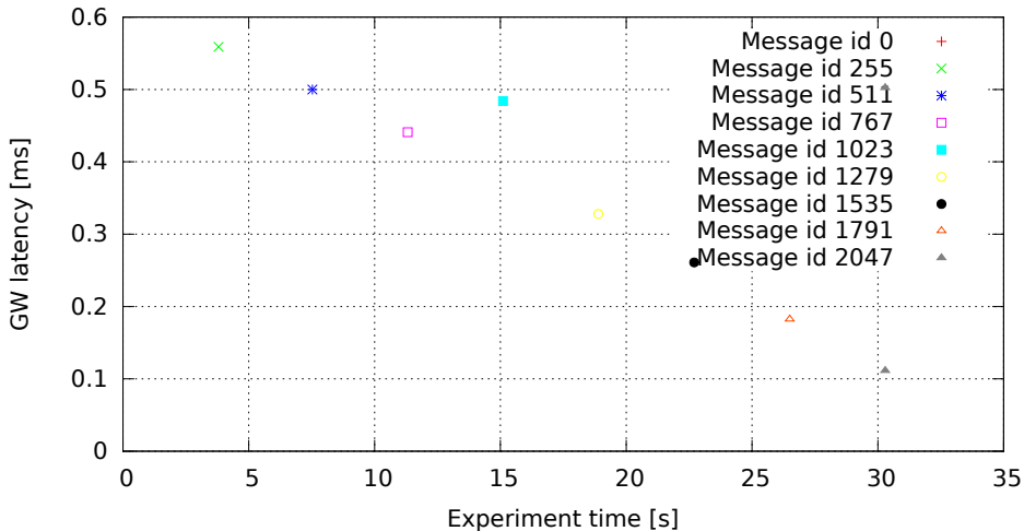
2048 GW rules (one per id, mask 0x7FF), no modifications (GW kernel 3.4.33-rt47-00004-gc58c9ae, Traffic 50, Load none)
