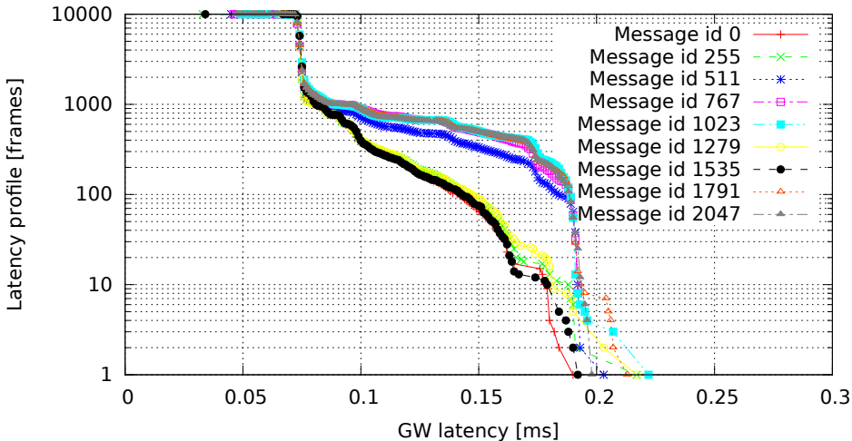
2048 GW rules (one per id, mask C00007FF), no modifications (GW kernel 3.4.33-rt47-00004-gc58c9ae, Traffic 50, Load none)
