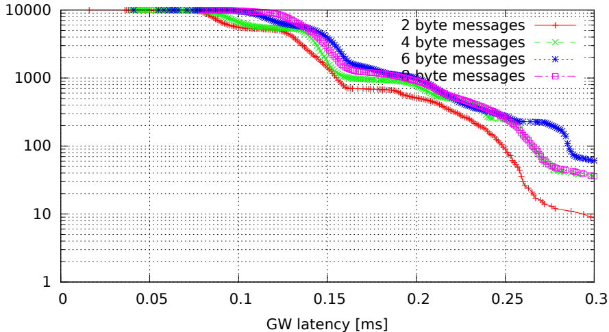
Single GW rule for all messages, no modifications (GW kernel 3.4.33-rt47-00004-gc58c9ae, Traffic 50, Load cpu)
