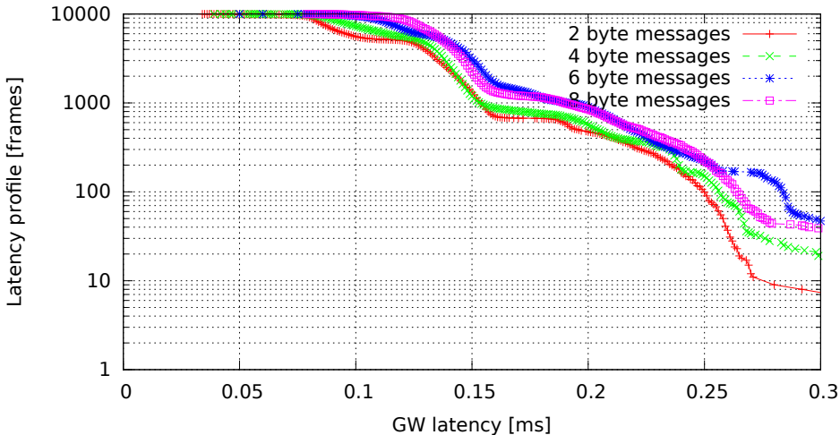
Single GW rule for all messages, no modifications, high (soft)irq task priority (GW kernel 3.4.33-rt47-00004-gc58c9ae, Traffic 50, Load cpu)
