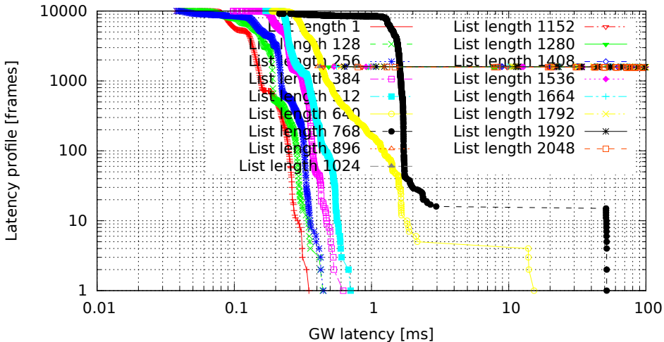
Different lengths of filter list, only the last one matches (GW kernel 3.4.33-rt47-00004-gc58c9ae, Traffic 50, Load cpu)
