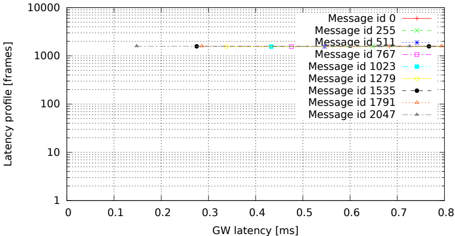
2048 GW rules (one per id, mask 0x7FF), no modifications (GW kernel 3.4.33-rt47-00004-gc58c9ae, Traffic 50, Load cpu)
