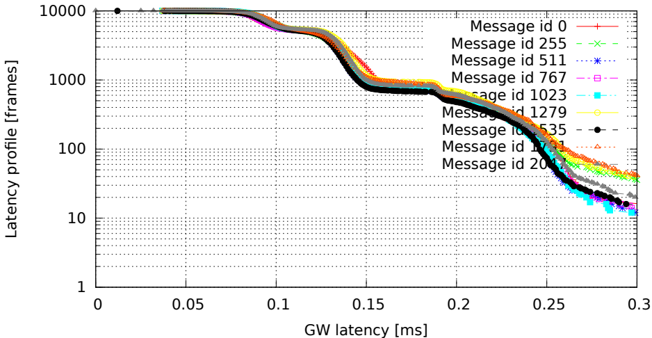
2048 GW rules (one per id, mask C00007FF), no modifications (GW kernel 3.4.33-rt47-00004-gc58c9ae, Traffic 50, Load cpu)
