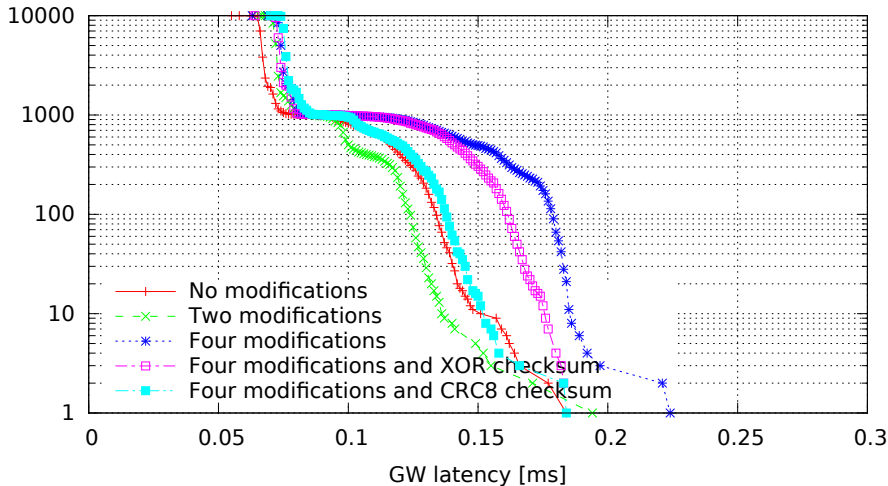
Single GW rule for all messages with modifications, 8 byte messages (GW kernel 3.0.7-rt20-00008-g0c18035, Traffic onetime, Load none)
