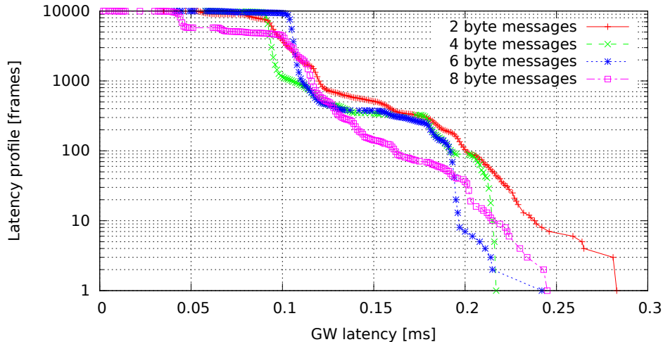
Single GW rule for all messages, no modifications (GW kernel 3.0.7-rt20-00008-g0c18035, Traffic flood, Load none)
