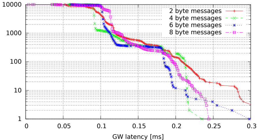
Single GW rule for all messages, no modifications, high (soft)irq task priority (GW kernel 3.0.7-rt20-00008-g0c18035, Traffic flood, Load none)
