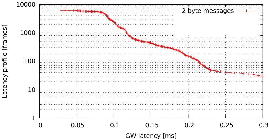
Single GW rule for all messages, no modifications, high (soft)irq task priority (GW kernel 3.0.7-rt20-00008-g0c18035, Traffic flood, Load eth)
