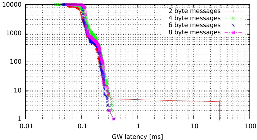
Single GW rule for all messages, no modifications (GW kernel 3.0.7-rt20-00008-g0c18035, Traffic flood, Load cpu)
