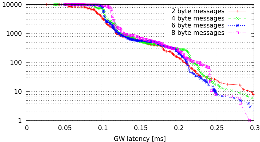
Single GW rule for all messages, no modifications, high (soft)irq task priority (GW kernel 3.0.7-rt20-00008-g0c18035, Traffic flood, Load cpu)
