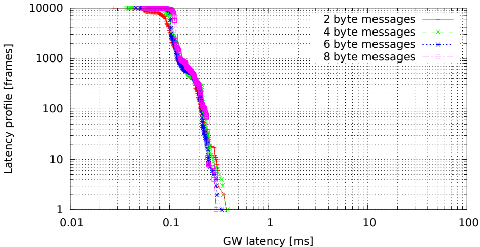
Single GW rule for all messages, no modifications, high (soft)irq task priority (GW kernel 3.0.7-rt20-00008-g0c18035, Traffic flood, Load cpu)
