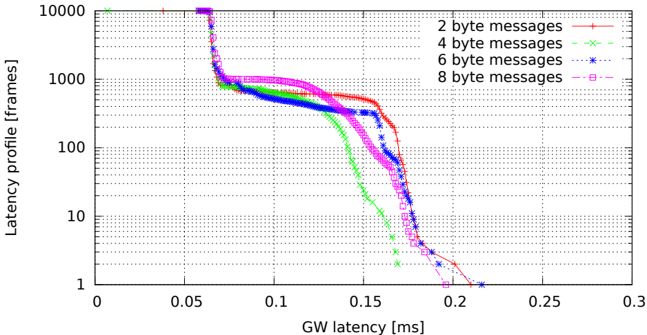
Single GW rule for all messages, no modifications, high (soft)irq task priority (GW kernel 3.0.4-rt14-00008-gb2052fd, Traffic oneatatime, Load none)
