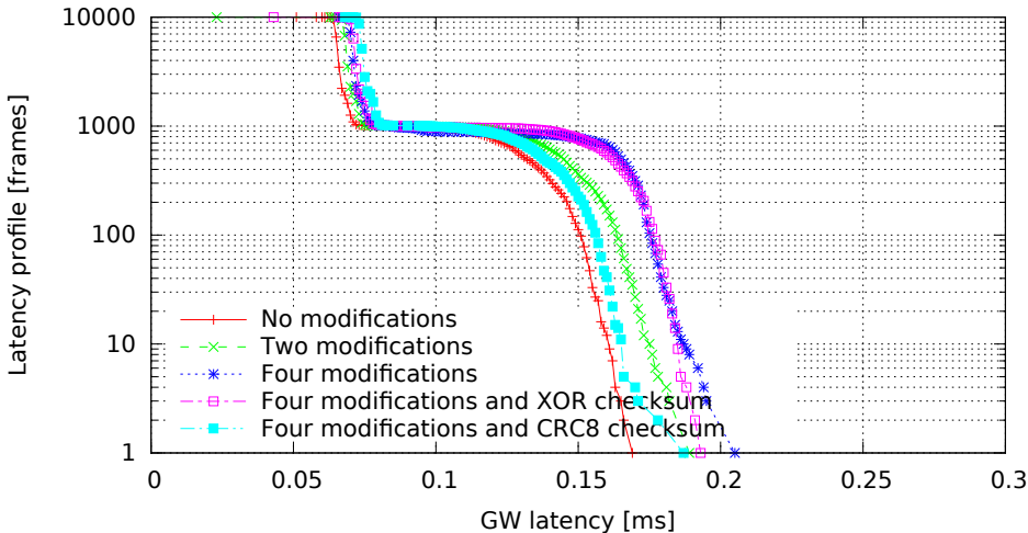
Single GW rule for all messages with modifications, 8 byte messages (GW kernel 3.0.4-rt14-00008-gb2052fd, Traffic onetatime, Load none)
