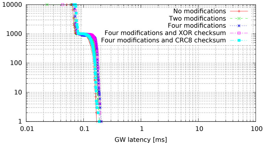
Single GW rule for all messages with modifications, 8 byte messages (GW kernel 3.0.4-rt14-00008-gb2052fd, Traffic onetatime, Load none)
