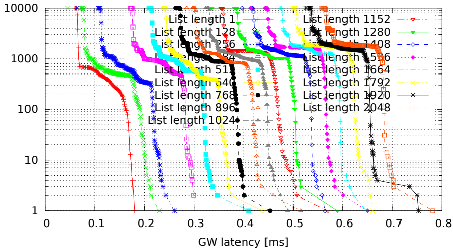
Different lengths of filter list, only the last one matches (GW kernel 3.0.4-rt14-00008-gb2052fd, Traffic oneatatime, Load none)
