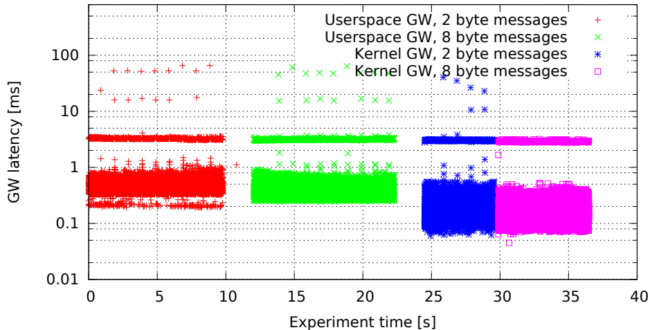
Single GW rule for all messages, no modifications (GW kernel 3.0.4-rt14-00008-gb2052fd, Traffic oneatatime, Load eth)
