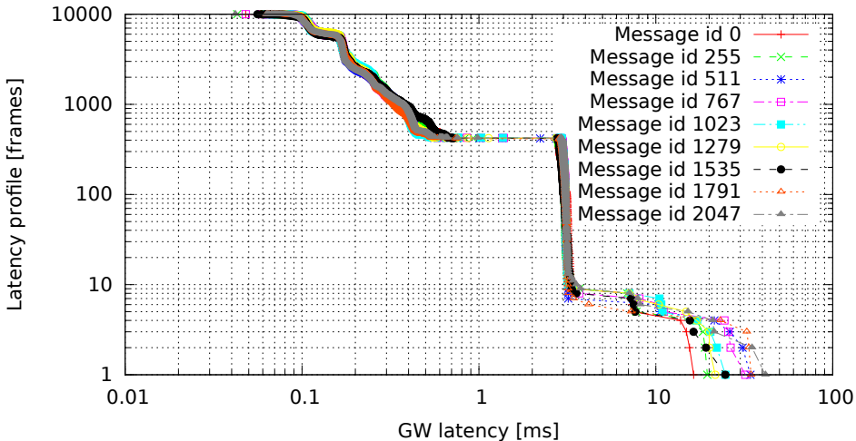
2048 GW rules (one per id, mask C00007FF), no modifications (GW kernel 3.0.4-rt14-00008-gb2052fd, Traffic onetotime, Load eth)
