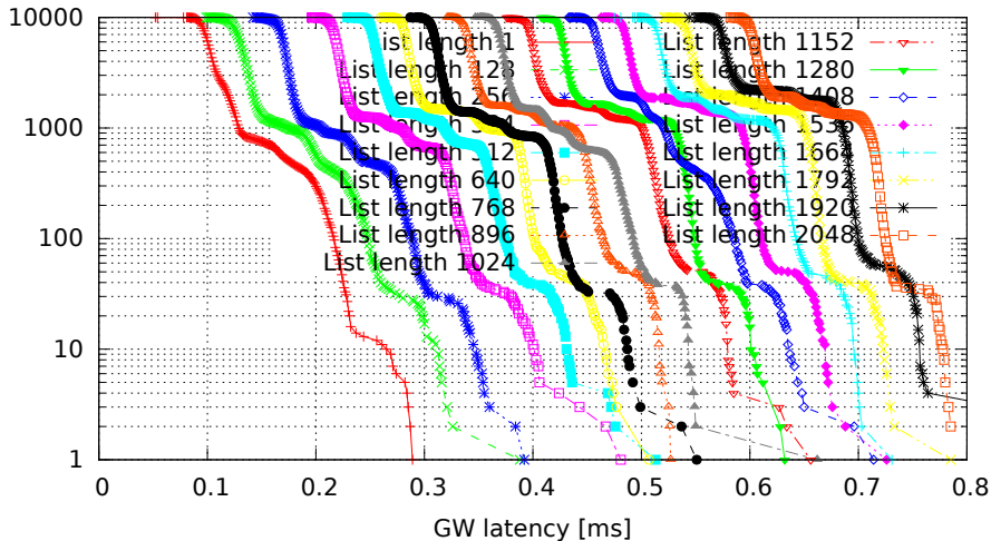
Different lengths of filter list, only the last one matches (GW kernel 3.0.4-rt14-00008-gb2052fd, Traffic oneatatime, Load cpu)
