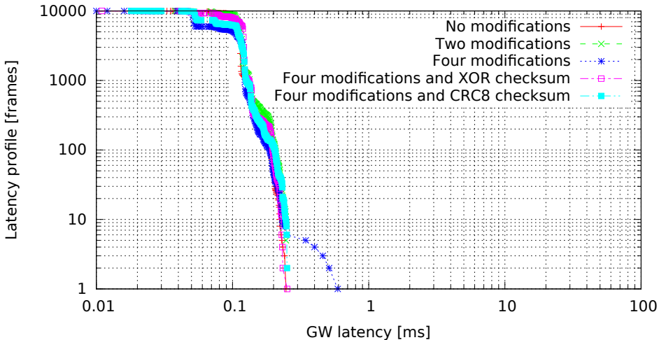
Single GW rule for all messages with modifications, 8 byte messages (GW kernel 3.0.4-rt14-00008-gb2052fd, Traffic flood, Load none)
