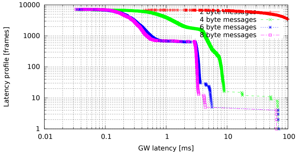
Single GW rule for all messages, no modifications (GW kernel 3.0.4-rt14-00008-gb2052fd, Traffic flood, Load eth)
