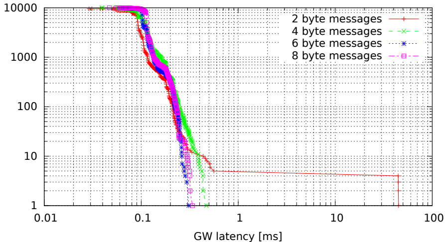
Single GW rule for all messages, no modifications (GW kernel 3.0.4-rt14-00008-gb2052fd, Traffic flood, Load cpu)
