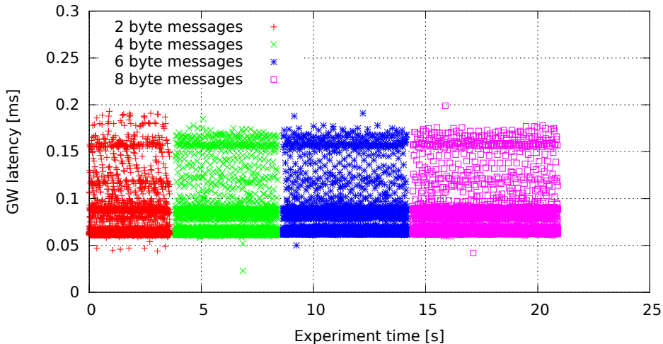
Single GW rule for all messages, no modifications, high (soft)irq task priority (GW kernel 3.0.4-rt14-00008-gb2052fd, Traffic 50, Load none)
