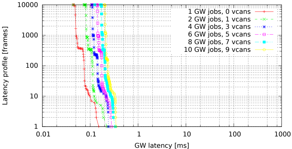
Chained GWs on multiple VCAN interfaces (GW kernel 3.0.4-00007-g1c8c373, Traffic oneatatime, Load none)
